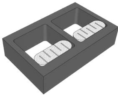
CMU Half High Jamb Unit with Icon® Inserts* (*special order item)
