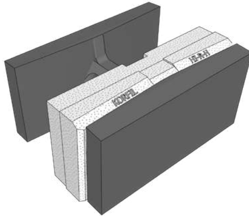
12×8×16 Spec-Thermal® HI-R-H Unit Fully Grouted Wall Assemblies
