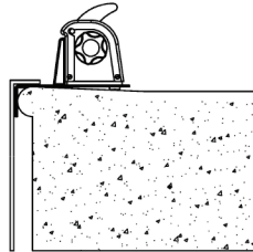
BULLNOSE COPING *REQUIRES P/N 143081-C-L
