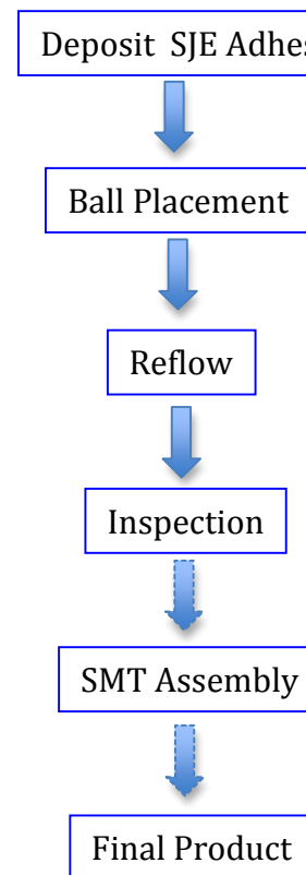
Fig.1 (b) Ball bumping using solder joint encapsulant (SJE) Adhesive
