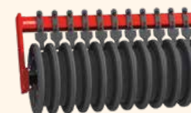
FARMFLEX-roller Ø 586 mm with scrapers without comb harrow
