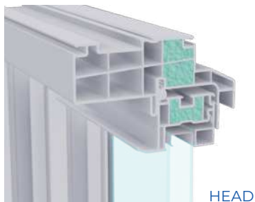
HEAD
