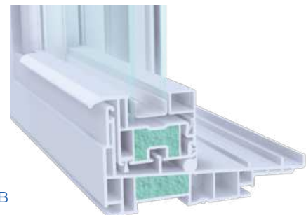
SILL
