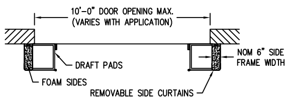
SECTION THRU PLAN
