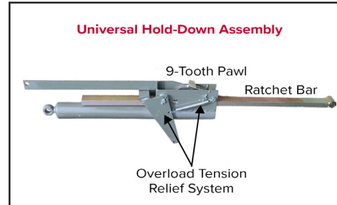
Components of hold-down system: 9-tooth pawl, ratchet bar and tension relief chain and system.
