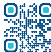
Telemedicine app
