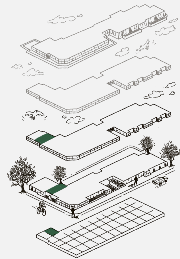
Basement Level
