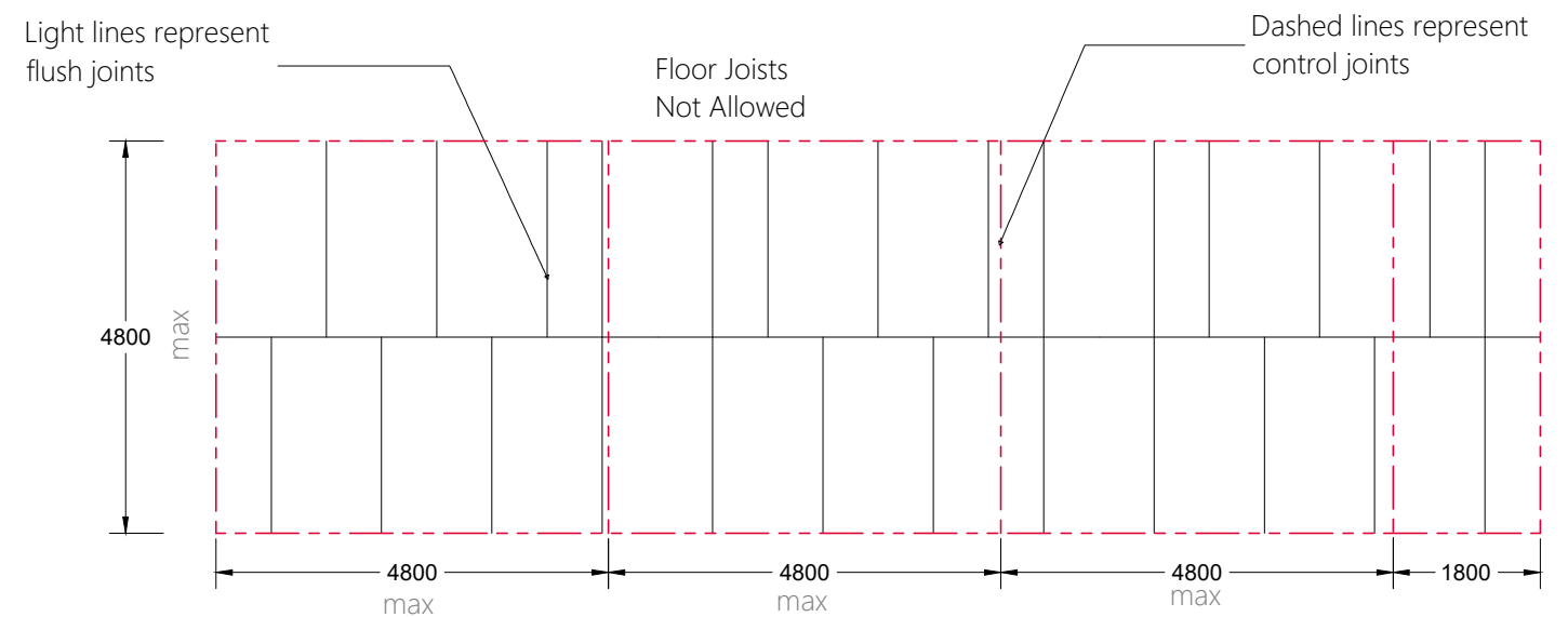
Typical control joint setout - Flush horizontal joint
