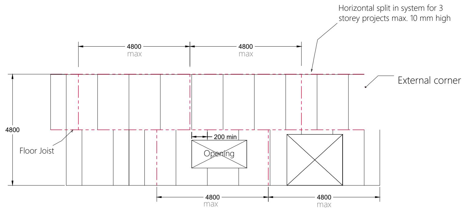
Typical control joint setout - Horizontal control joint
