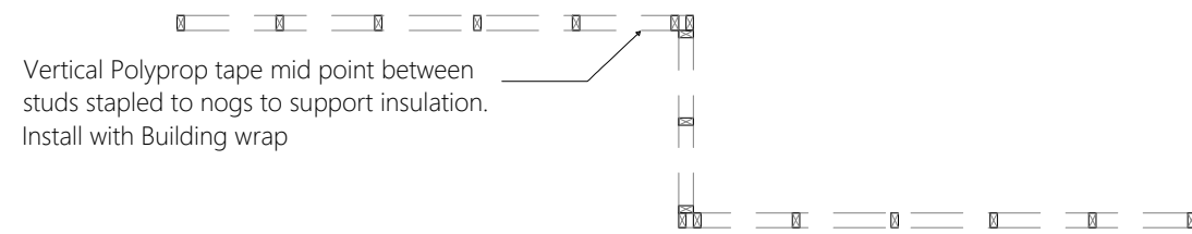
Typical Wall Panel Plan
