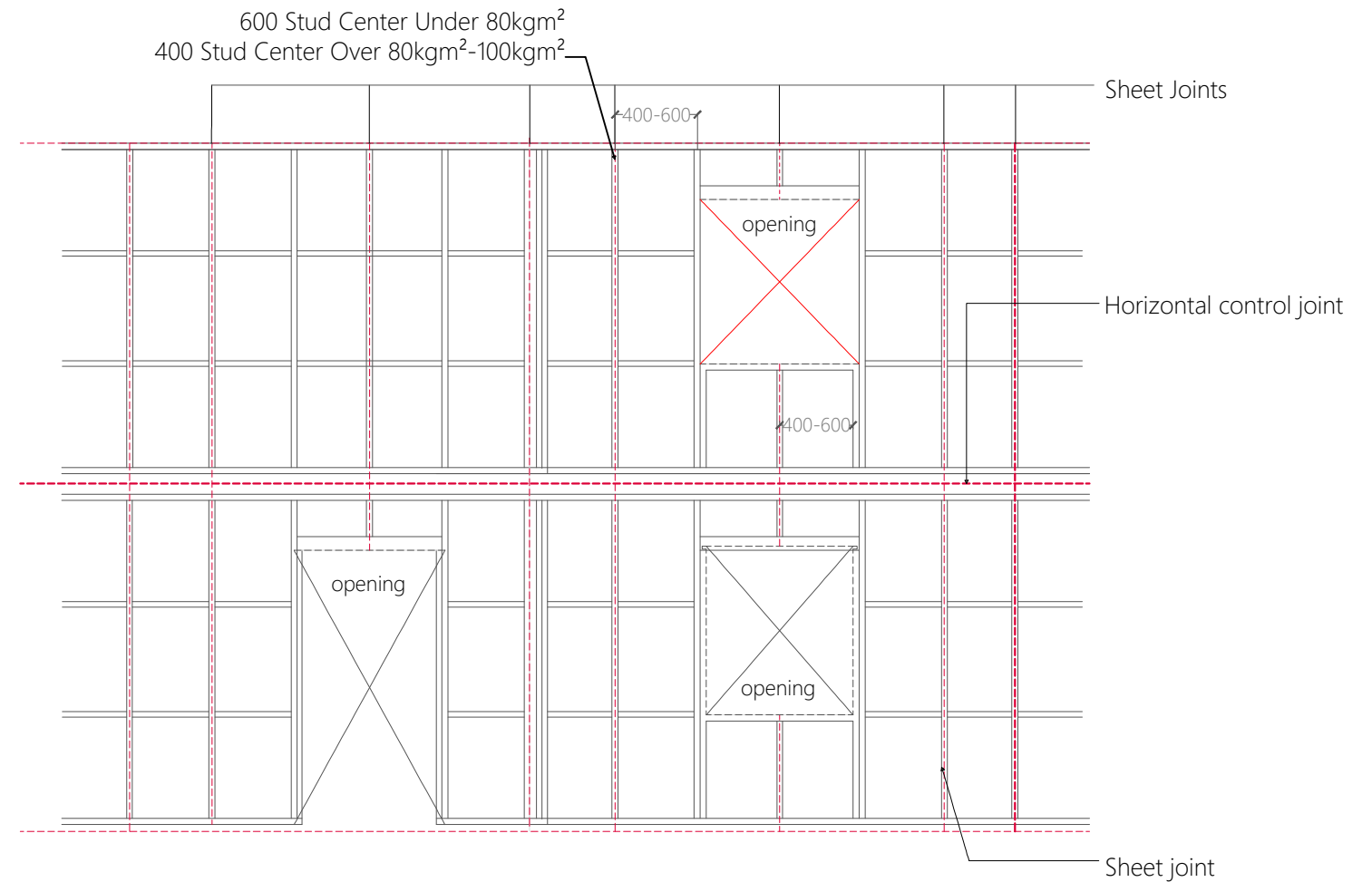
Typical Wall Panel Elevation (Framing Layout)
