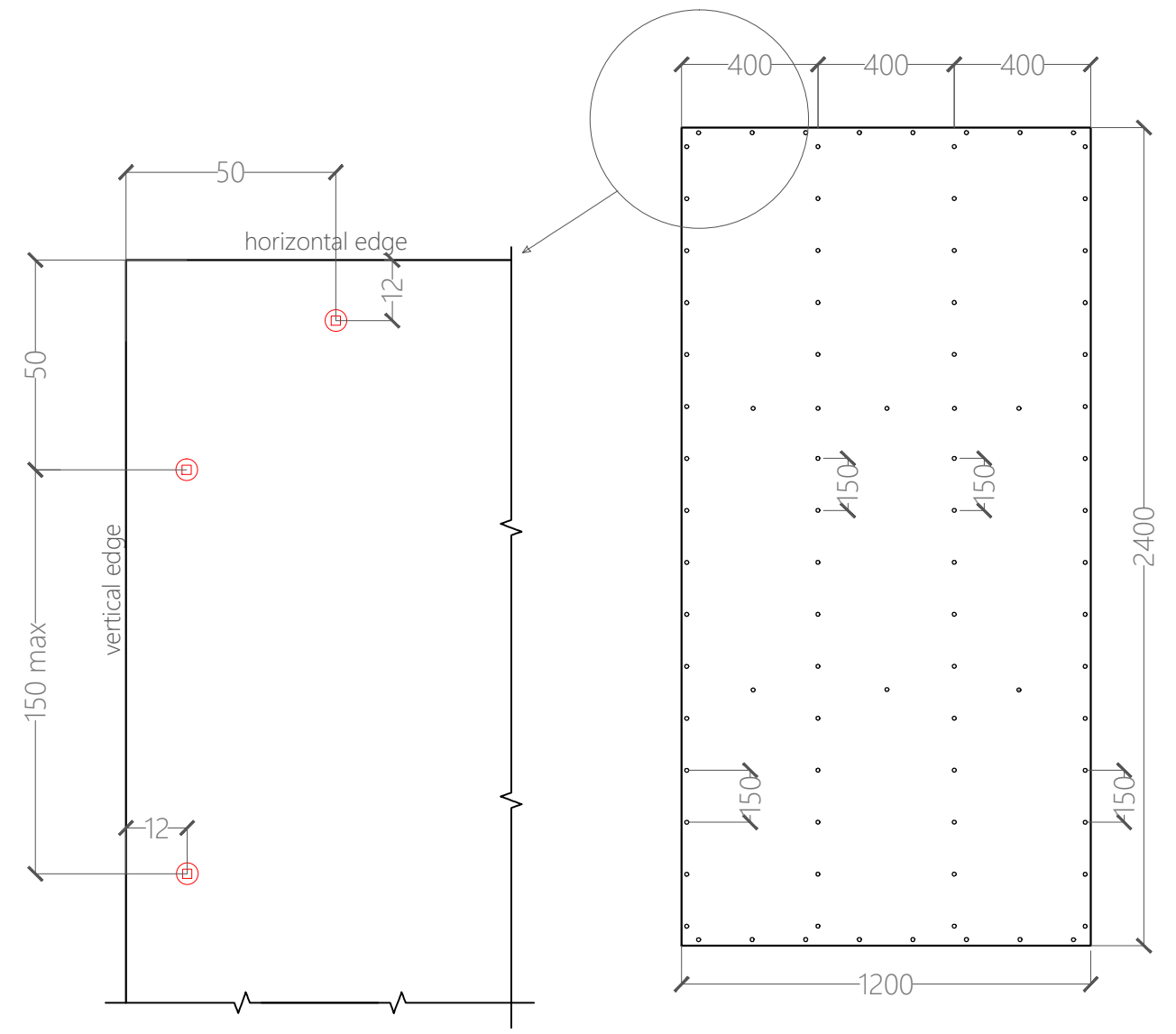
Screw fixing distances from sheet edge
