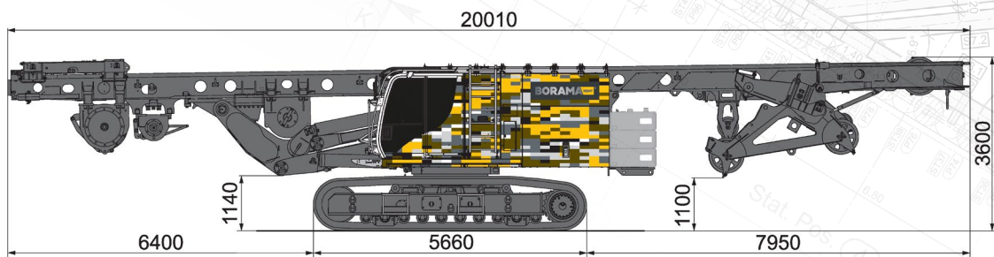
Transport position
