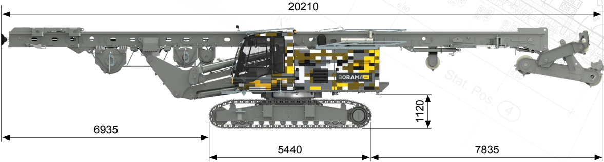
Transport position
