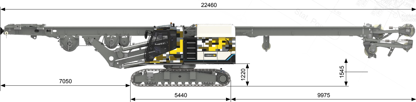
Transport position
