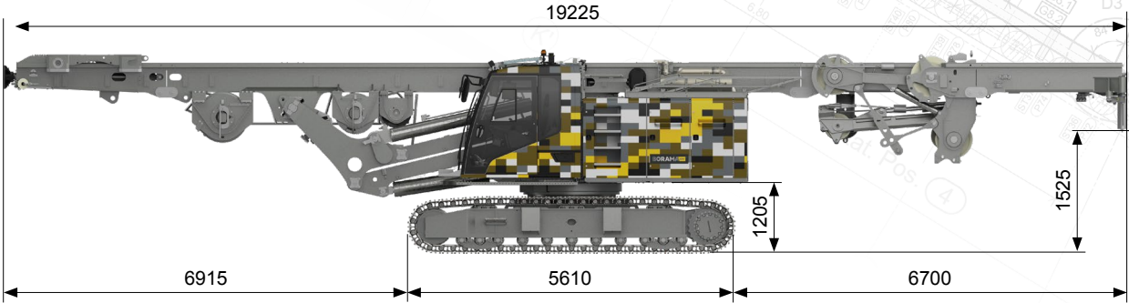
Transport position
