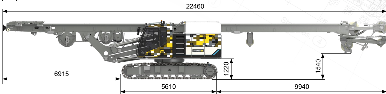
Transport position
