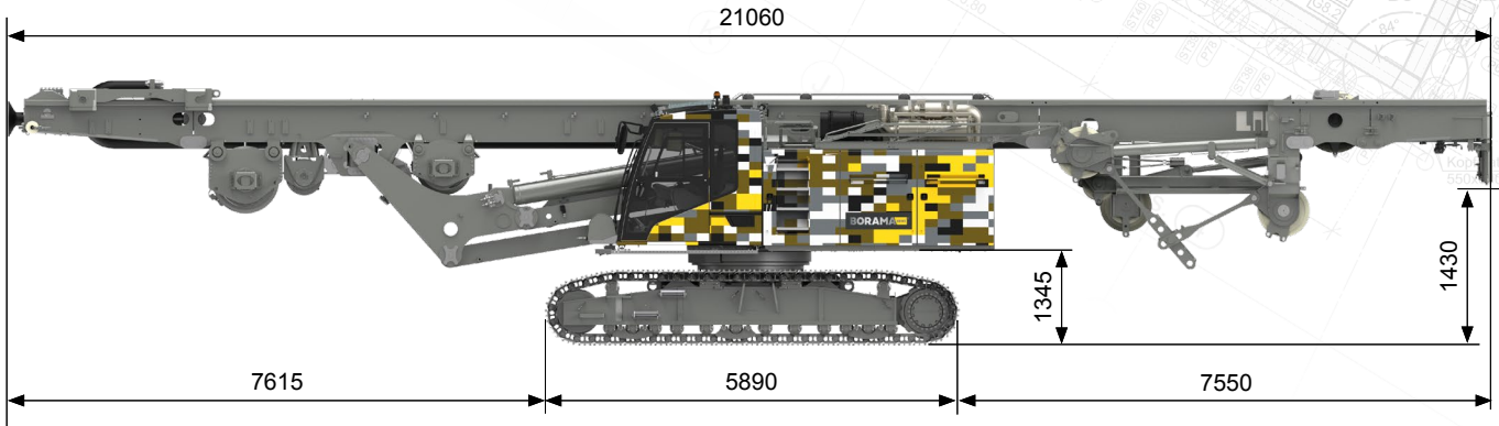
Transport position
