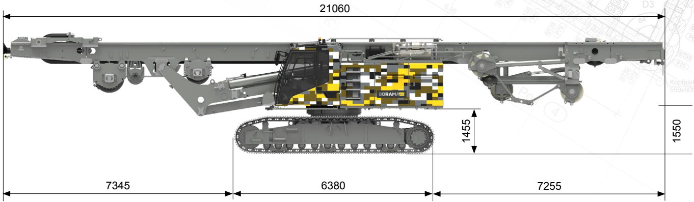
Transport position
