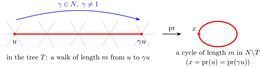
Figure 3: Theorem 2.5: a cycle downstairs lifts to a walk upstairs between two vertices of the same orbit. Large girth therefore follows from showing that every \gamma \neq 1 moves every vertex far.
