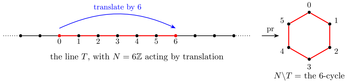
Figure 2: Quotienting the line by translations by 6 produces a 6-cycle. The red path from 0 to its translate 6 projects onto the cycle.
