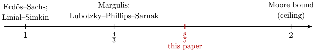
Figure 9: Known values of the constant c in \text{girth}(G) \geq c \log_{d-1} n - O(1) .
