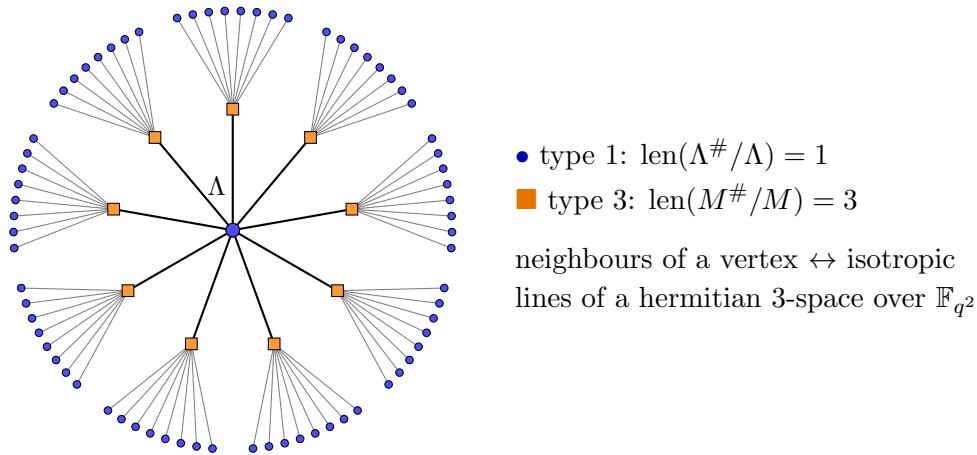
Figure 6: The neighbourhood of a type-1 vertex \Lambda of T for q = 2 : its q^3 + 1 = 9 neighbours have type 3, and each of them has q^3 = 8 further neighbours.
