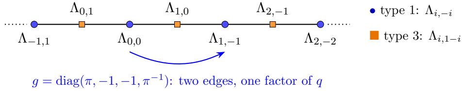
Figure 5: An apartment (a bi-infinite path) in T . Consecutive vertices of the same type are two edges apart.
