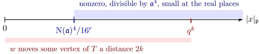
Figure 8: The certificate: the number x = \det(w - I) satisfies both bounds, so q^k \geq N(\mathfrak{a})^4/16^r .
