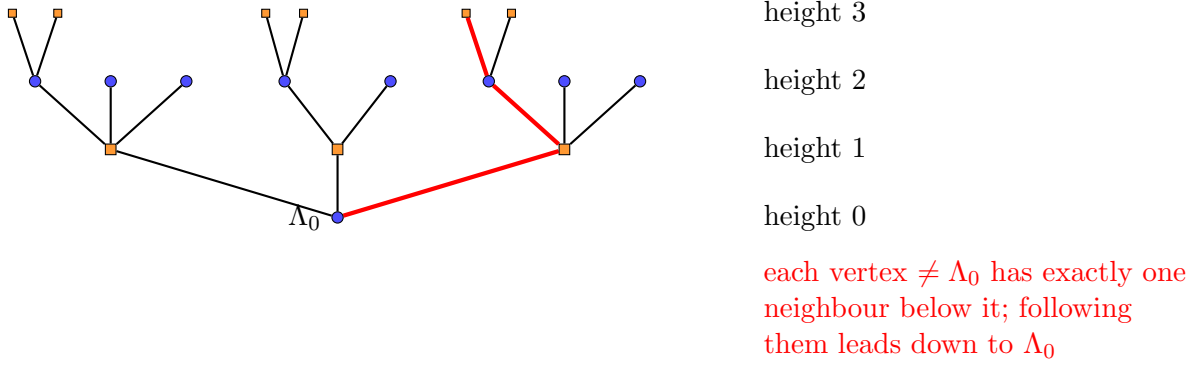
Figure 7: Heights (schematic, fewer branches drawn).
