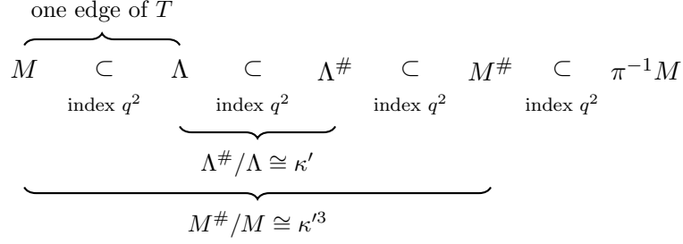
Figure 4: The lattices around an edge \{M, \Lambda\} of T , with t(M) = 3 and t(\Lambda) = 1 . Each step is an inclusion of index q^2 .
