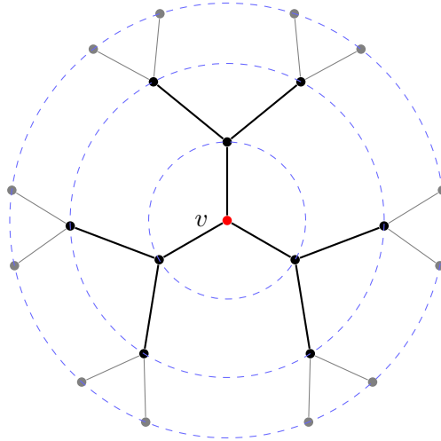
Figure 1: If the girth exceeds 2r , the ball of radius r around any vertex is a tree with \approx (d-1)^r vertices (here d = 3 , r = 3 ). Hence n \gtrsim (d-1)^{g/2} .
