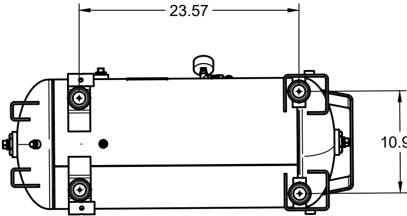
BOTTOM VIEW
