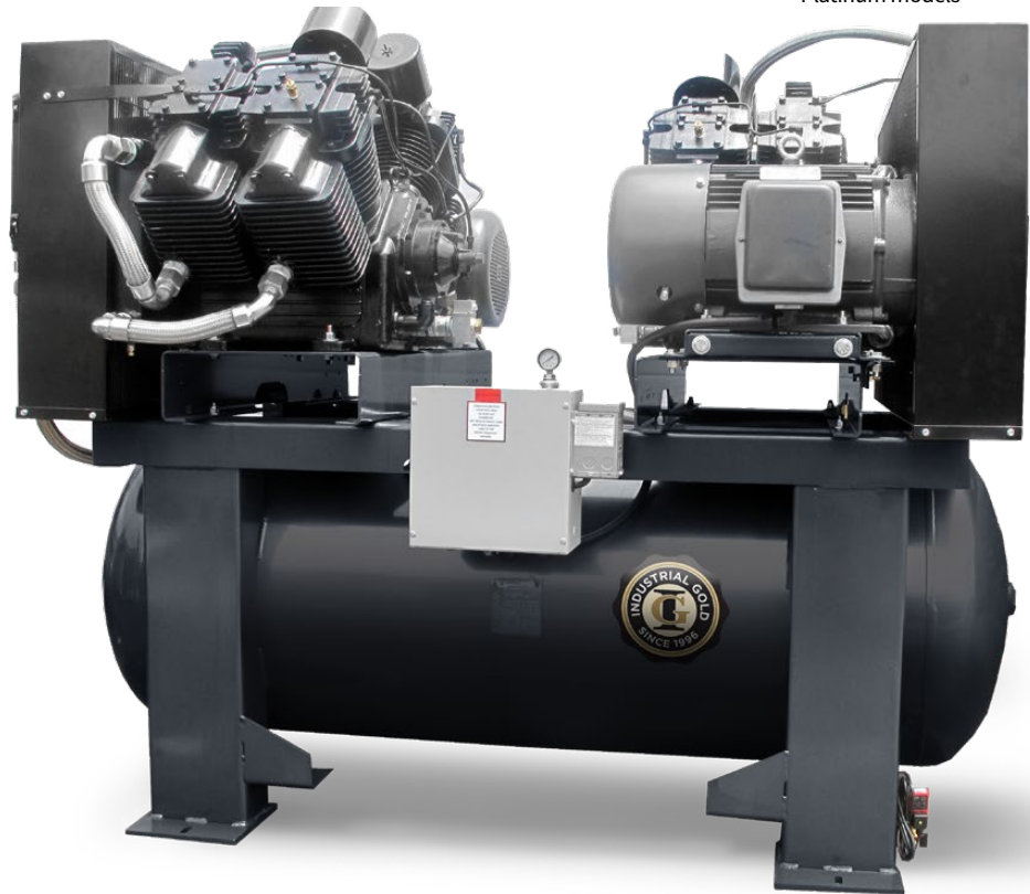
Air cooled after cooler on Platinum models
