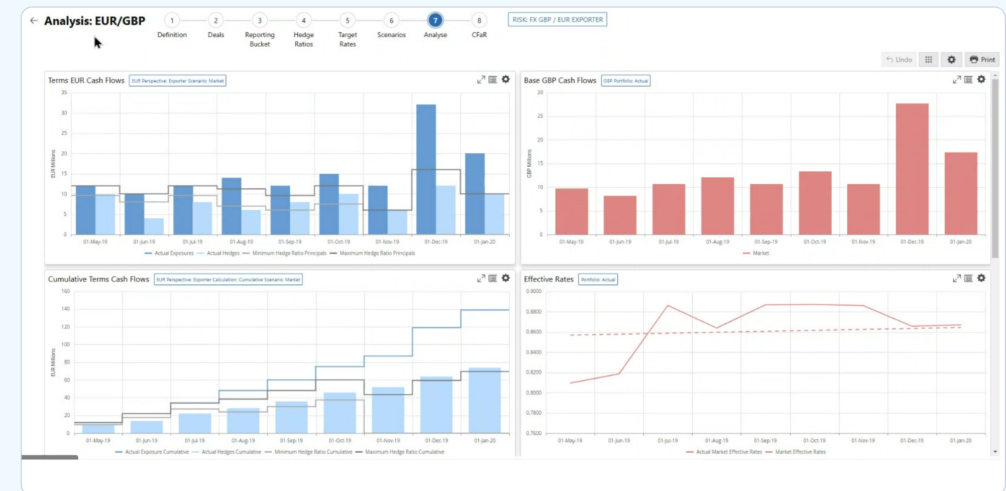
FX dashboard
