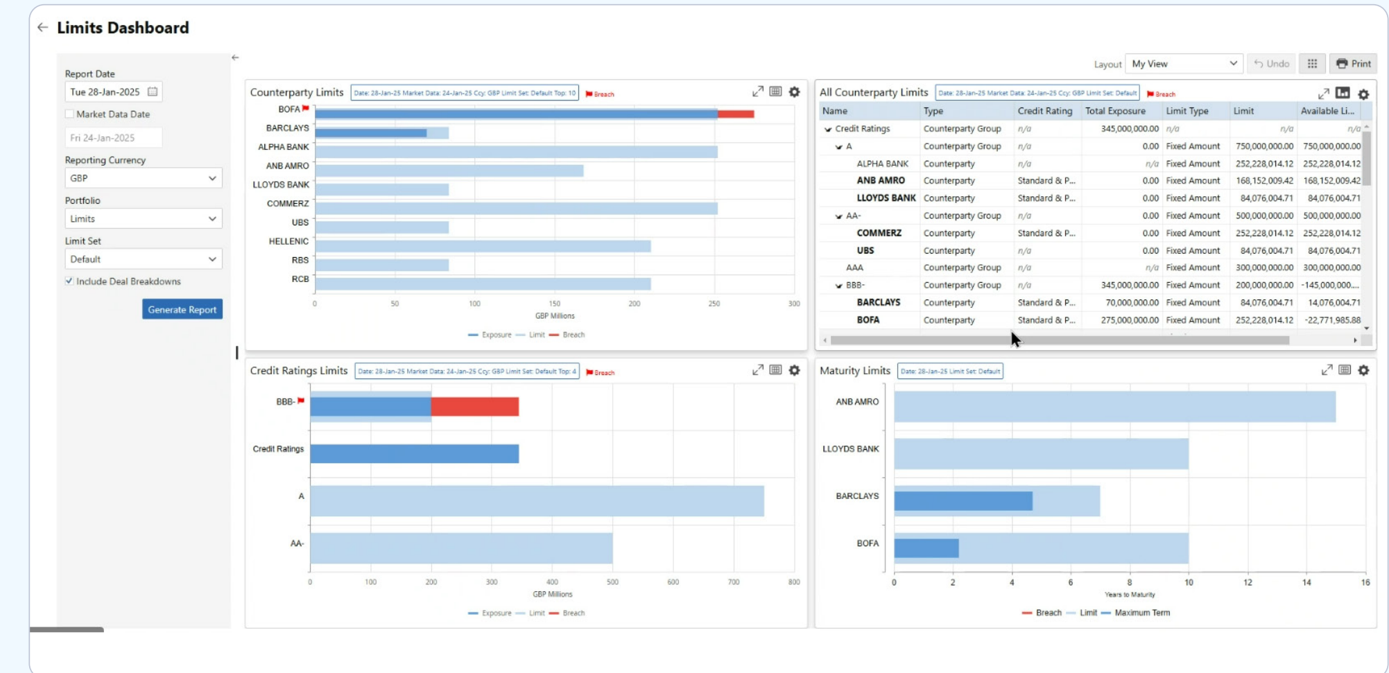
Limits dashboard
