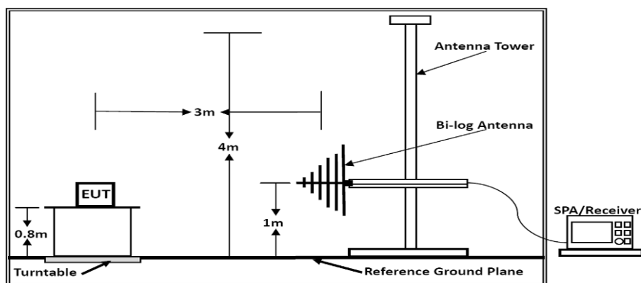
Below 1GHz
