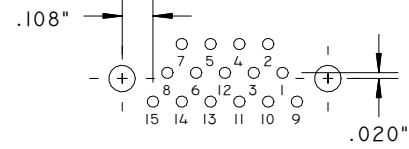
15 PIN
