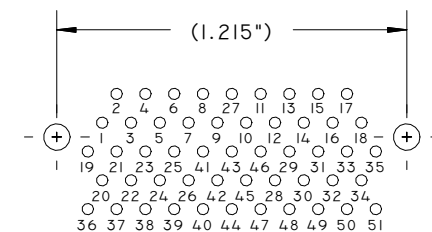
51 SOCKET
