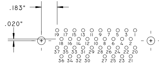
37 PIN
