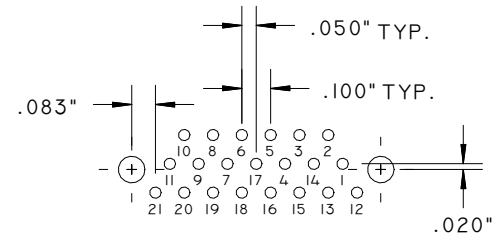
21 PIN
