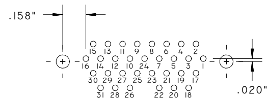
31 PIN
