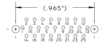
25 SOCKET
