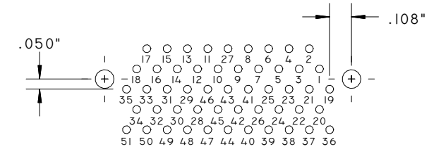
51 PIN
