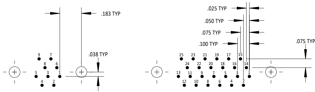
9 CONTACTS
