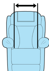
Seat Width 485mm (W)
