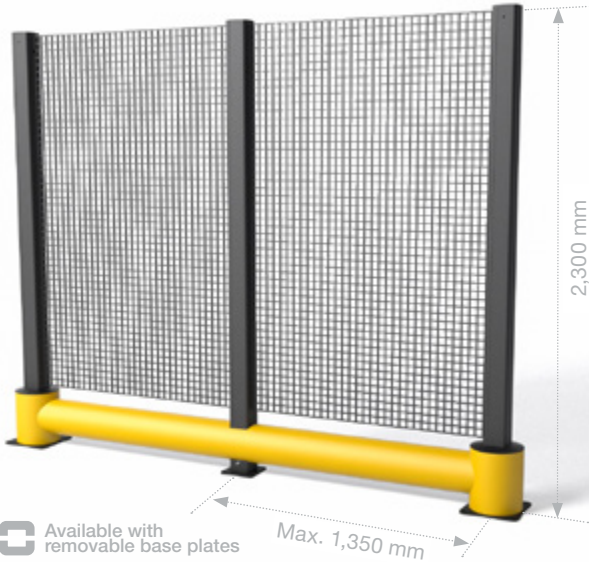
Available with removable base plates TB 260 PLUS FENCE 21.20 kJ
