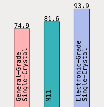
INTEGRATED ABSORPTION COEF. CENTERED AT 395nm (normalized)
