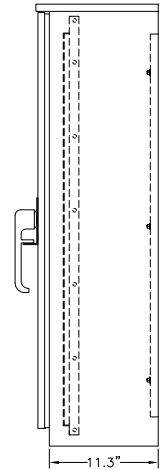
PANEL SIDE VIEW
