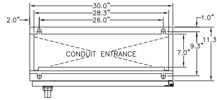
PANEL BASE PLAN
