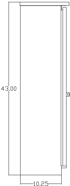
LEFT VIEW
