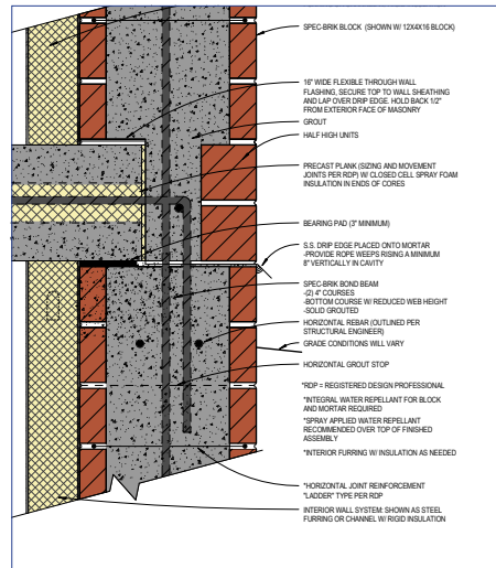
Figure 20. Pre-Cast Plank Option 4
