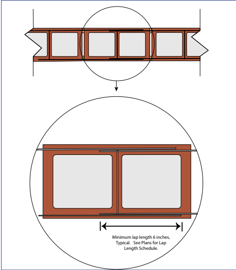
Figure 15. Joint Reinforcement
