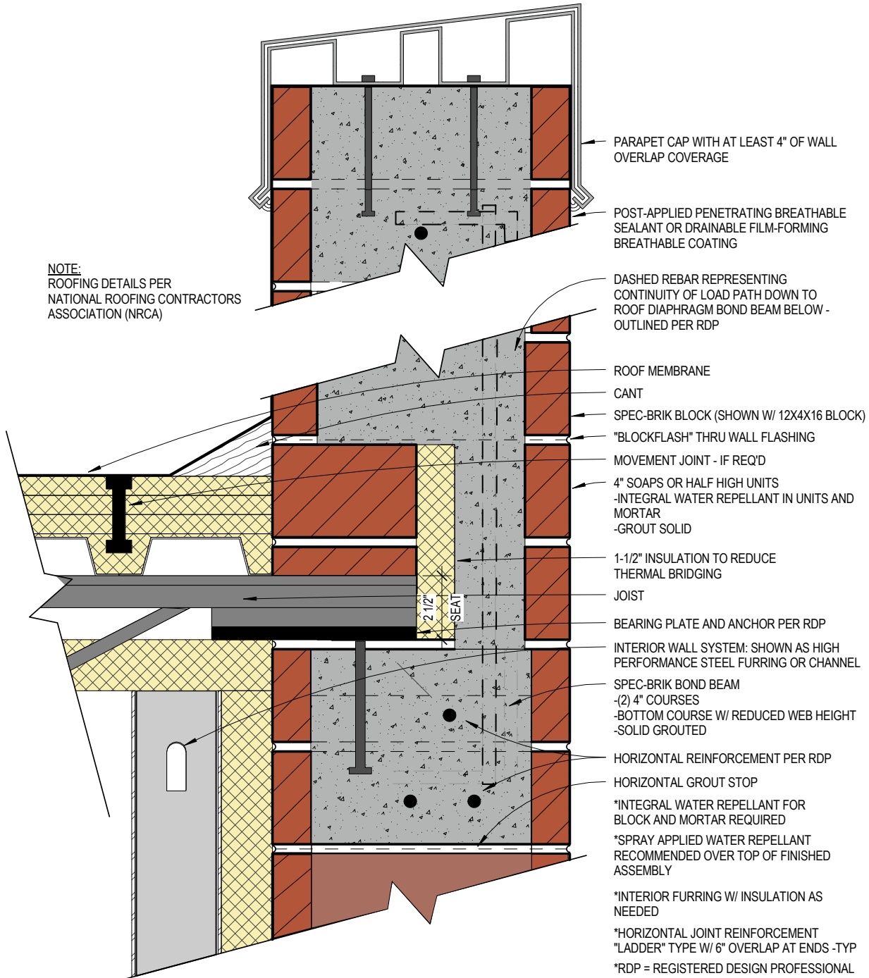
Figure 21. Roof Parapet
