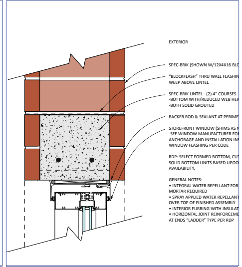
Figure 14. Lintel
