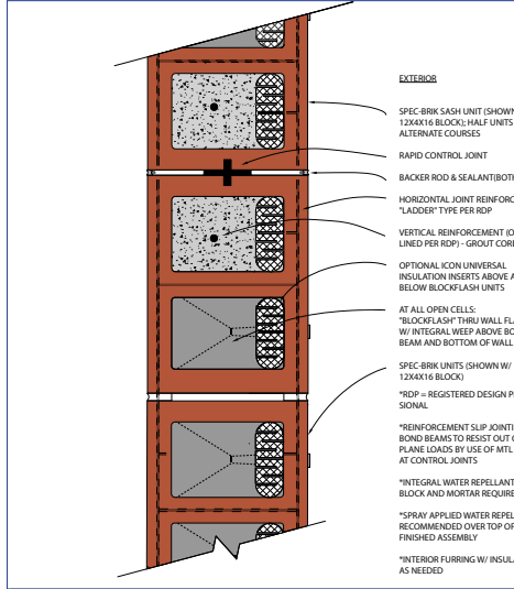
Figure 16. Movement Joint
