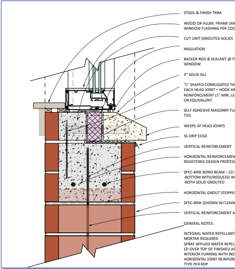
Figure 12. Window Sill
