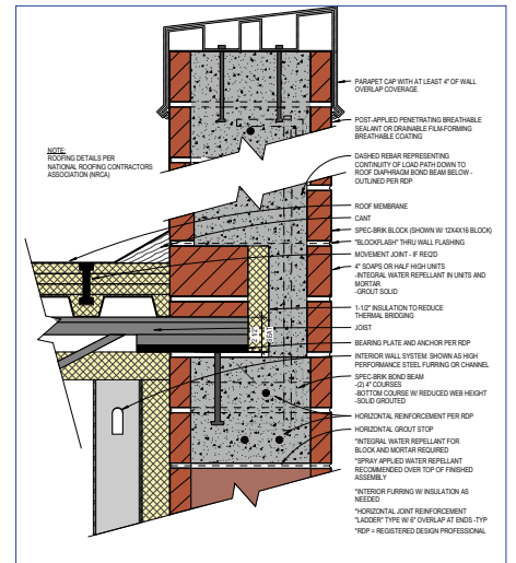
Figure 21. Roof Parapet
