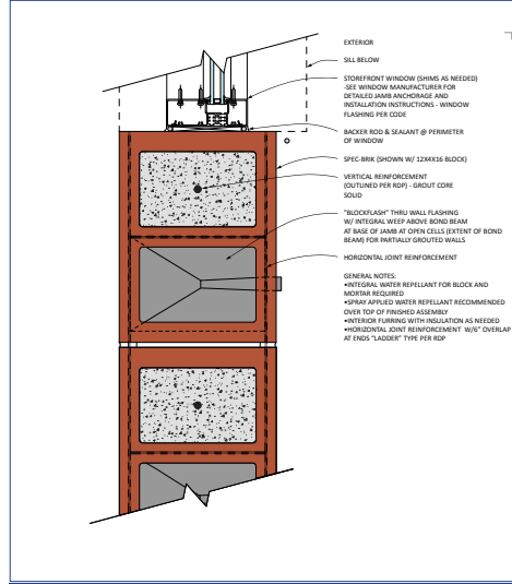
Figure 13. Window Jamb
