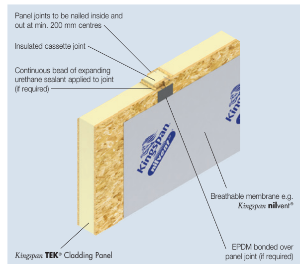
Figure 5 – Vertical Panel Junction with Insulated Cassette Joint
