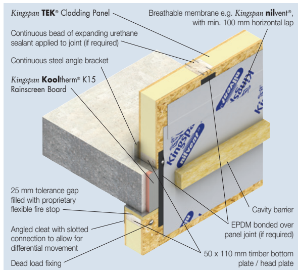
Figure 3 – 'In-board', Fixing Inside the Structural Frame
