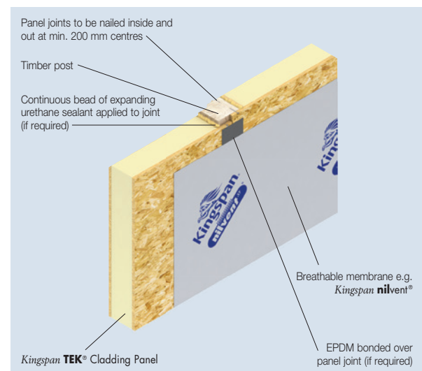
Figure 6 – Vertical Panel Junction with Timber Post
