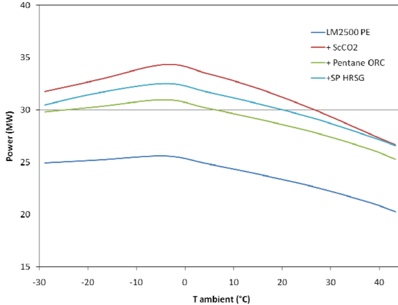
Figure 4: System performance model for an Echogen utility scale heat engine integrated to a LM2500 power generation turbine compared to competing waste heat recovery technologies.
