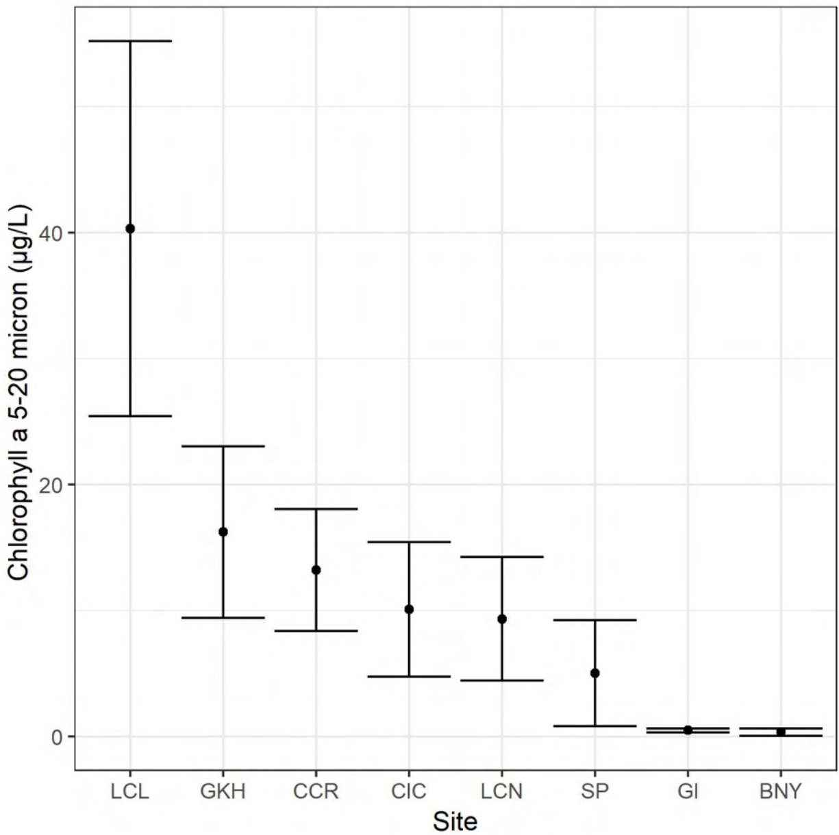
Figure 41. Average chlorophyll a concentration for particles between 5 and 20 µm in 2018 at Brooklyn Navy Yard (BNY), Canarsie Community Reef (CCR), Coney Island Community Reef (CIC), Governors Island EcoDock (GI), Great Kills Harbor (GKH), Lemon Creek Lagoon (LCL), Lemon Creek Nursery (LCN), and Sunset Park Community Reef (SP). Error bars represent 95% confidence intervals.
