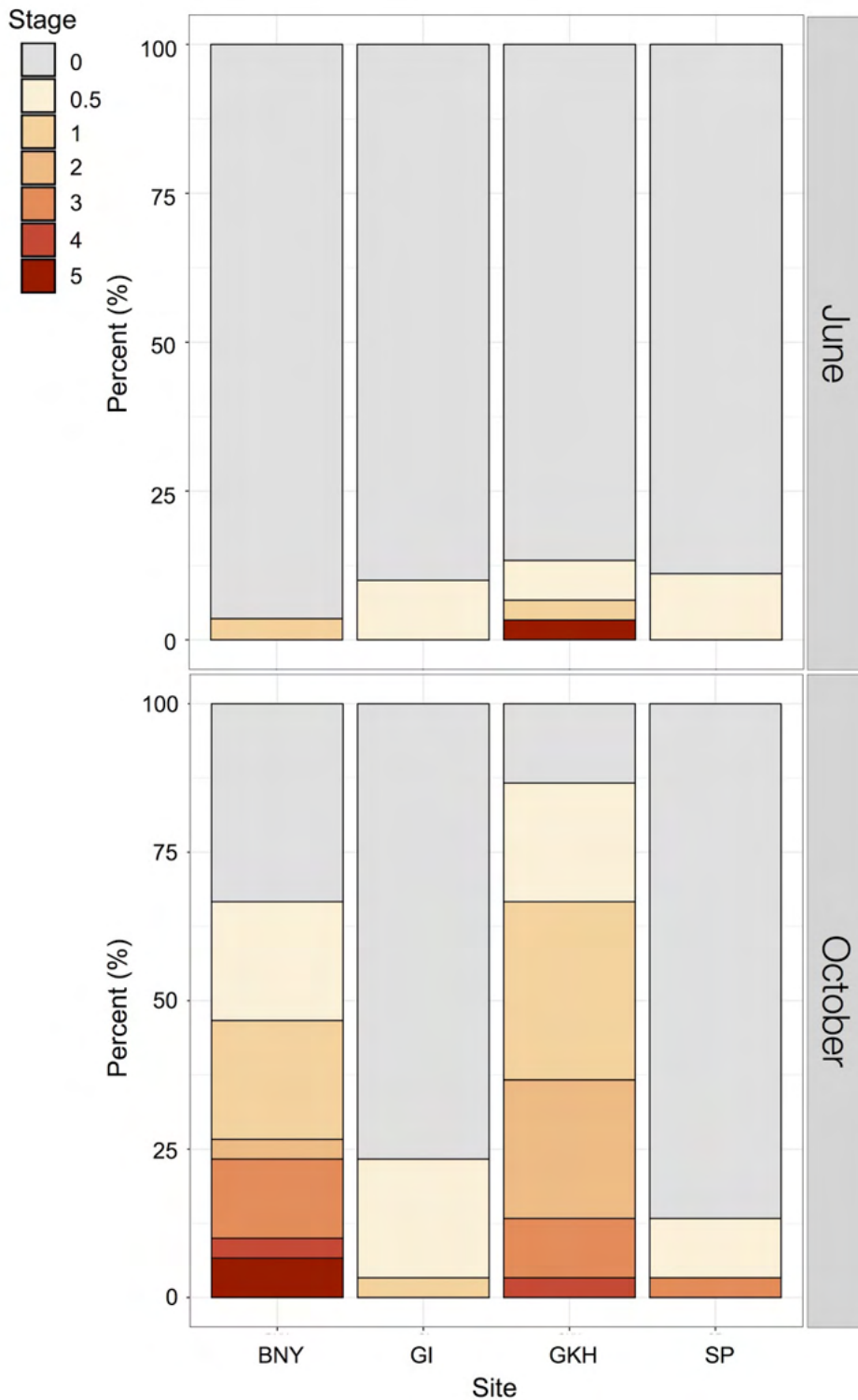
Figure 24. Dermo ( P. marinus ) prevalence and intensity in oysters from Brooklyn Navy Yard (BNY), Governors Island EcoDock (GI), Great Kills Harbor (GKH) MBSOS07152015 cohort installed in 2016, and the Sunset Park (SP) Community Reef in June and October 2018 (n = 30 oysters per site, except n = 27 for SP in June). Oysters with intensities ranking 3 or higher are considered to be lethally infected.
