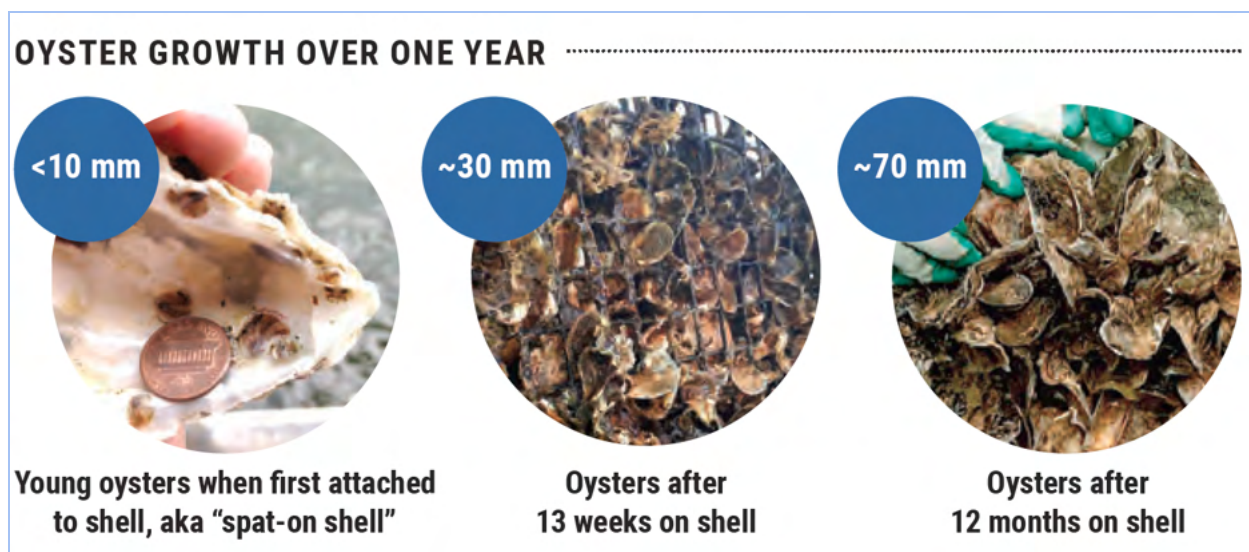
Figure 7. These photos show oyster growth in the first year of restoration at sites with fast growth.
