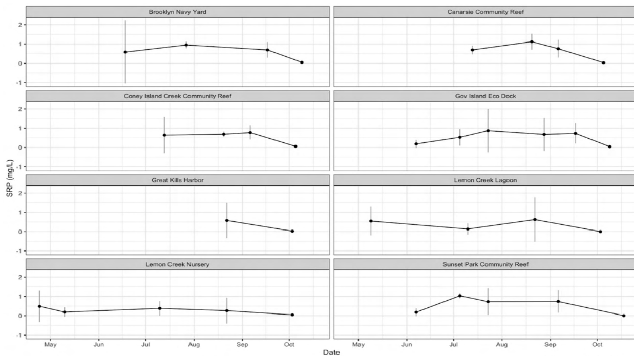
Figure 43. Soluble reactive phosphorus concentrations at Brooklyn Navy Yard, Canarsie Community Reef, Coney Island Creek Community Reef, Governors Island EcoDock, Great Kills Harbor, Lemon Creek Lagoon, Lemon Creek Nursery, and Sunset Park Community Reef in 2018. Error bars represent 95% confidence intervals.
