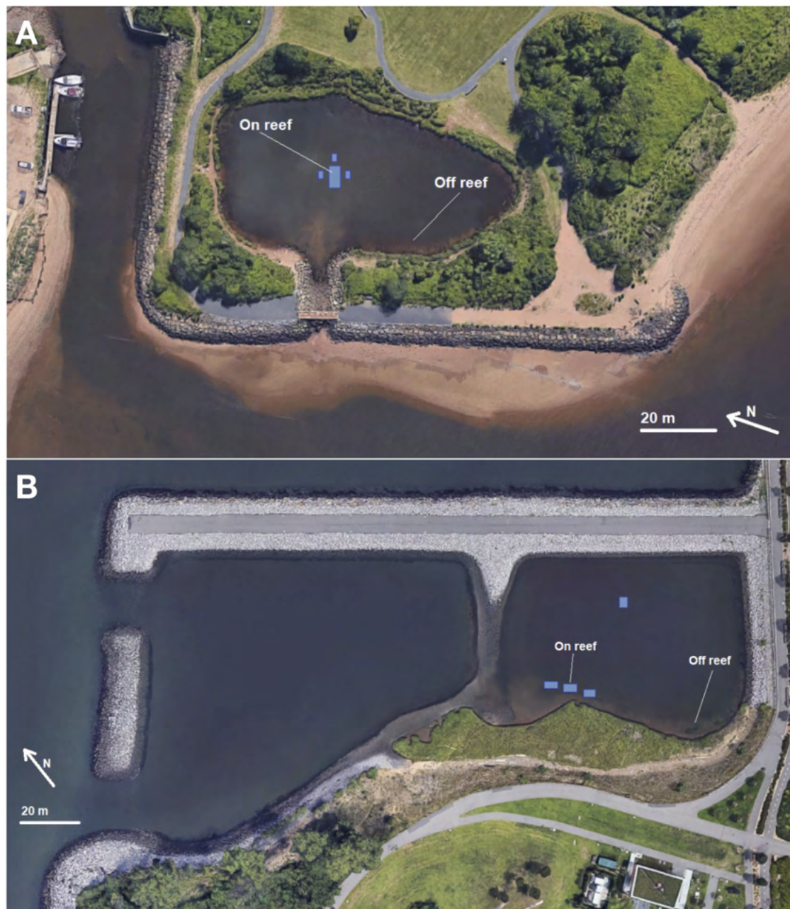
Figure 46. Aerial view of biodiversity study sites at (A) Lemon Creek Lagoon and (B) Sunset Park Community Reef at Bush Terminal Park. Blue polygons indicate approximate size and location of oyster restoration projects.
