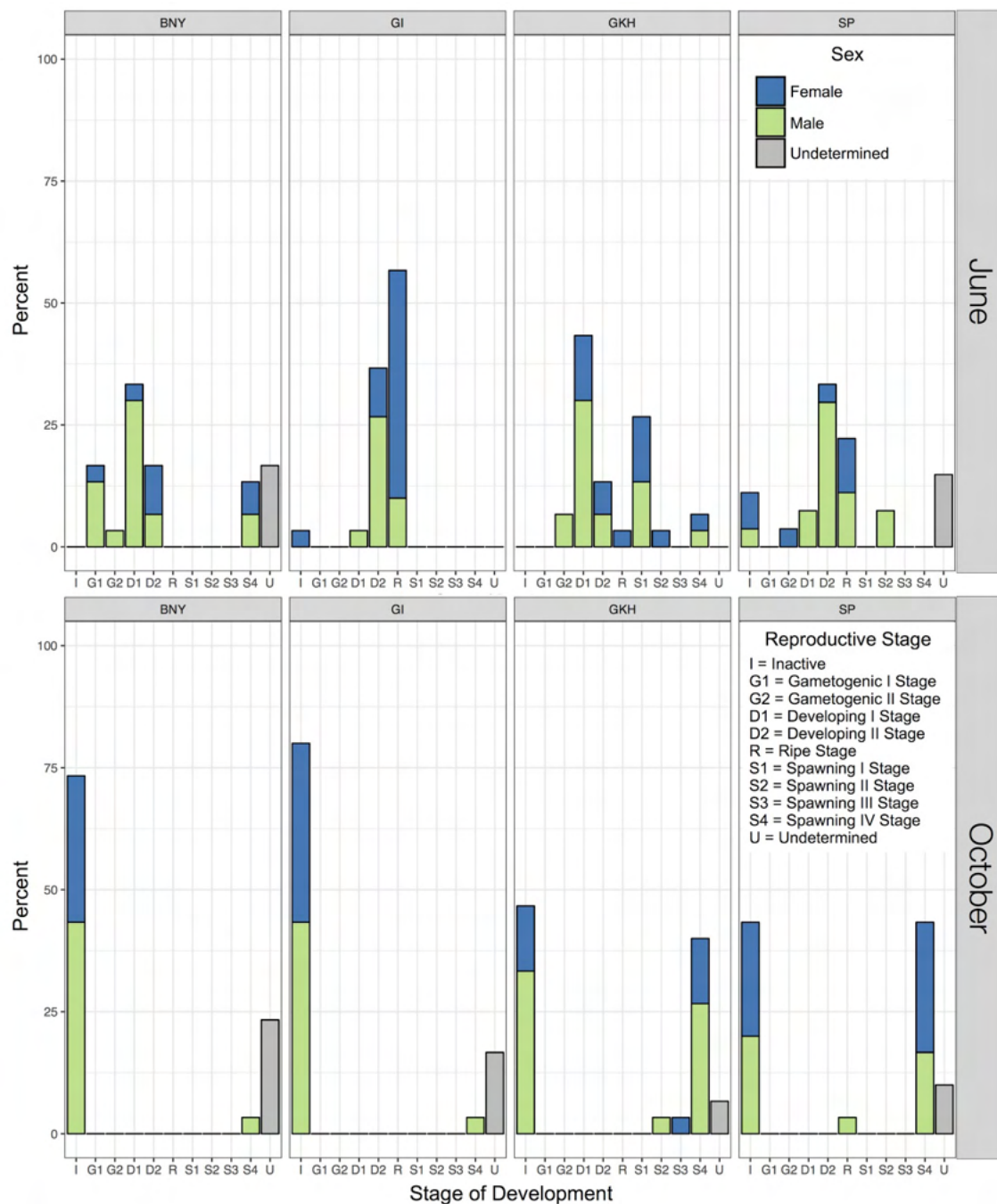
Figure 26. Stage of reproductive development and sex of oysters from Brooklyn Navy Yard (BNY), Governors Island EcoDock (GI), and Great Kills Harbor (GKH) MBSOS07152015 cohort (installed in 2016) in June and October 2018 (n = 30 oysters from each site). Sexual maturity generally increases from left to right, but see Table 6 for a full description of the reproductive stages.
