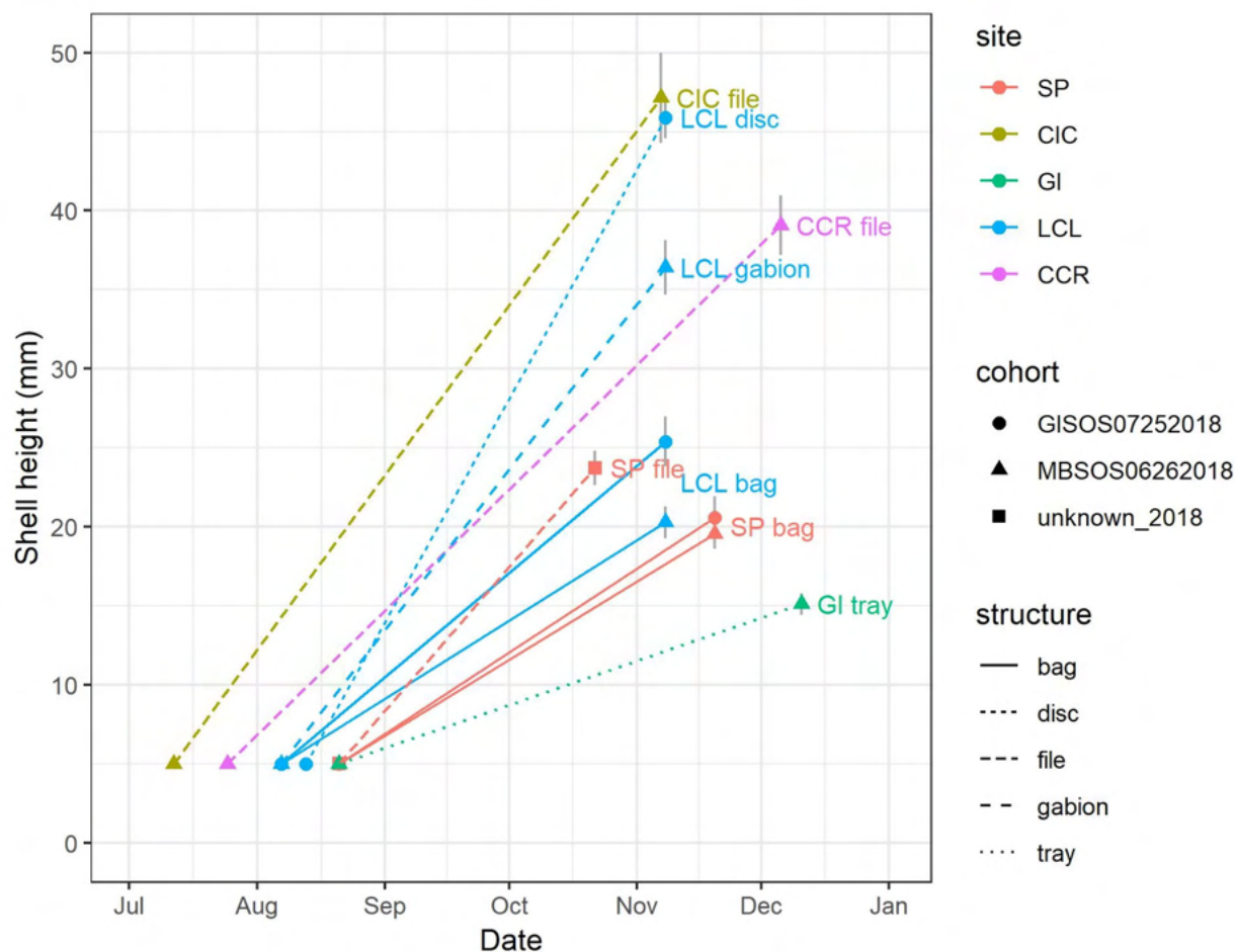
Figure 9. Oyster shell height over time for oysters installed in 2018 at Canarsie Community Reef (CCR), Coney Island Creek (CIC), Governors Island EcoDock (GI), Lemon Creek Lagoon (LCL), and the Sunset Park (SP) Community Reef and bagged shell reef. Error bars indicate 95% confidence intervals. “unknown_2018” cohort is a mix of GISOS07252018 and MBSOS06262018.
