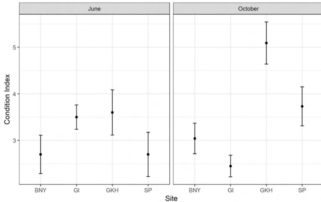
Figure 28. Condition index of oysters from Brooklyn Navy Yard (BNY), Governors Island EcoDock (GI), Great Kills Harbor (GKH) MBSOS07152015 cohort, and Sunset Park (SP) Community Reef in June and October (n = 30 oysters from each site, except n = 27 for SP and n = 28 for BNY in June). Error bars represent 95% confidence intervals.
