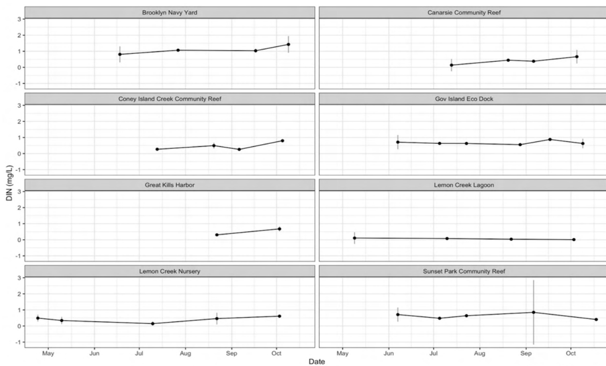
Figure 44. Dissolved inorganic nitrogen (the sum of nitrite, nitrate, and ammonium) concentrations at Brooklyn Navy Yard, Canarsie Community Reef, Coney Island Creek Community Reef, Governors Island EcoDock, Great Kills Harbor, Lemon Creek Lagoon, Lemon Creek Nursery, and Sunset Park Community Reef in 2018. Error bars represent 95% confidence intervals.
