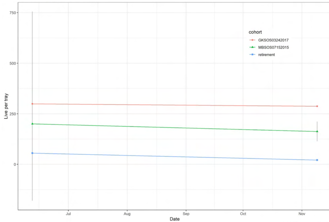
Figure 22. Oyster density (live per tray) in Super Trays at Great Kills Harbor changed little in 2018. Error bars represent 95% confidence intervals.
