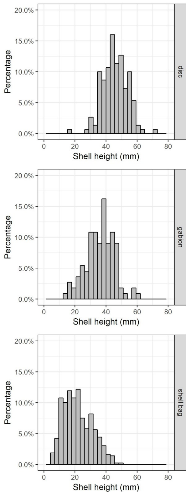
Figure 14. Size frequency distribution of live oyster shell heights on EConcrete® discs, gabions, and the bagged shell reef at Lemon Creek Lagoon in November 2018.
