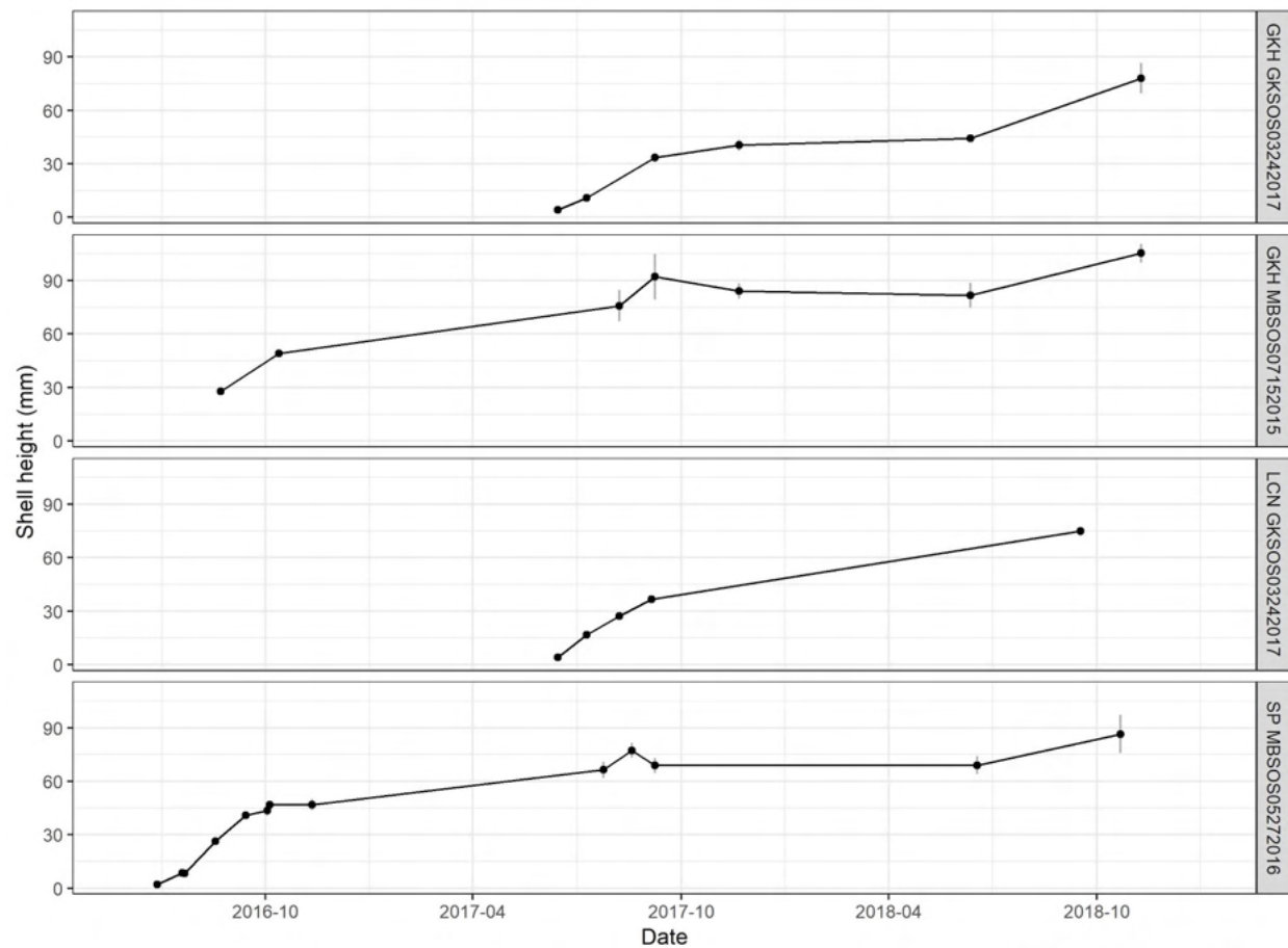
Figure 10. Oyster shell height over time for oysters installed prior to 2018 at Great Kills Harbor (GKH), Lemon Creek Nursery (LCN), and Sunset Park (SP) Community Reef. Error bars indicate 95% confidence intervals.
