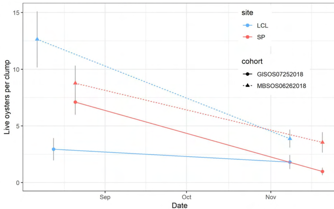
Figure 17. Oyster density (i.e., live oysters per clump) declined over time at bagged shell reefs at Lemon Creek Lagoon (LCL) and Sunset Park (SP) reef at Bush Terminal Park in 2018. Initial densities are measured in the hatchery within one week of deployment. Error bars represent 95% confidence intervals.
