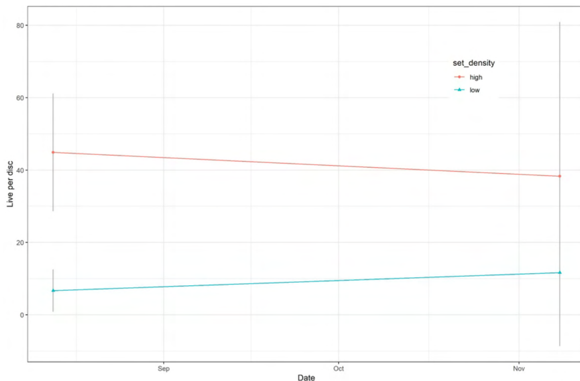
Figure 21. Oyster density (live per disc) on EConcrete® discs at the Lemon Creek Lagoon changed little in 2018. “set_density” indicates discs that were set with low or high densities of larvae in the Hatchery. Error bars represent 95% confidence intervals.
