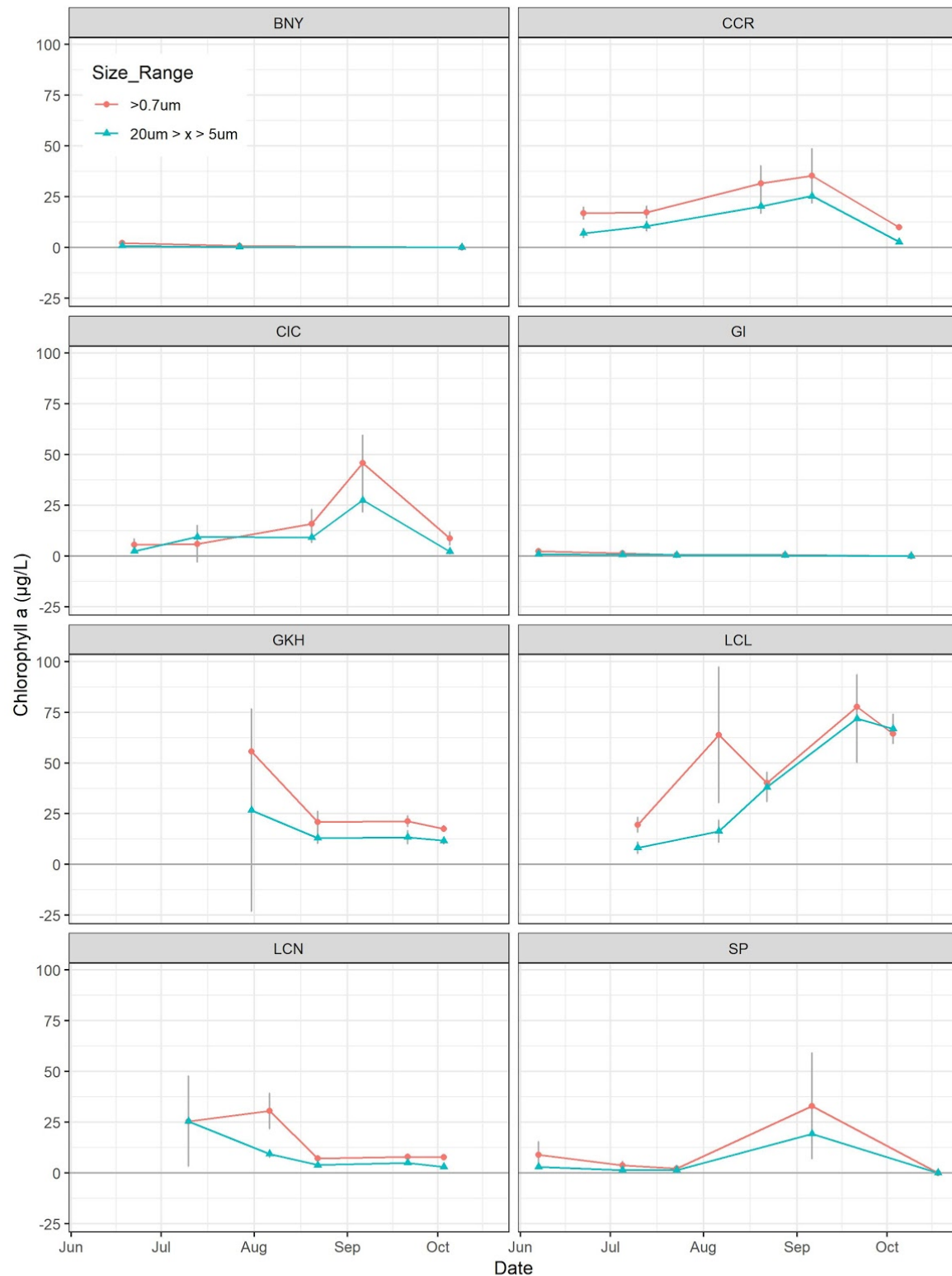
Figure 42. Chlorophyll a concentration for all particles >0.7 µm and particles between 5 and 20 µm at Brooklyn Navy Yard (BNY), Canarsie Community Reef (CCR), Coney Island Community Reef (CIC), Governors Island EcoDock (GI), Great Kills Harbor (GKH), Lemon Creek Lagoon (LCL), Lemon Creek Nursery (LCN), and Sunset Park Community Reef (SP). Error bars represent 95% confidence intervals.
