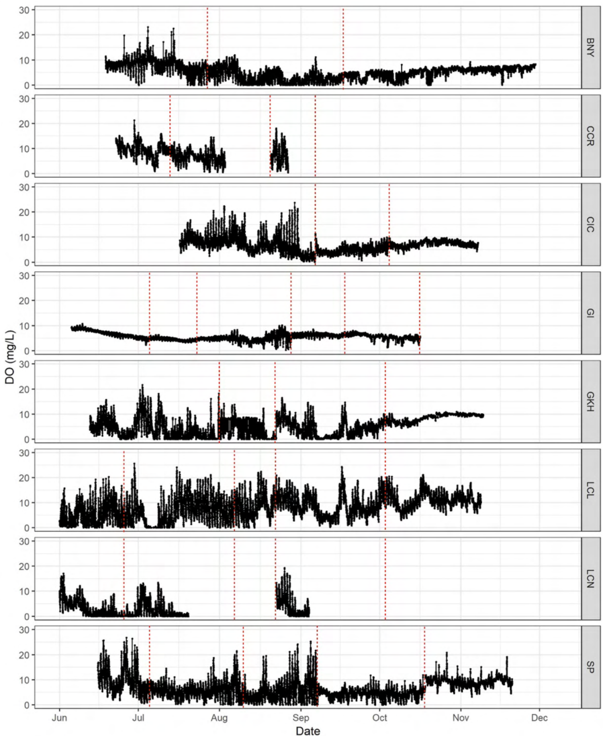
Figure 39. High-resolution (recorded every 15 minutes) dissolved oxygen data for Brooklyn Navy Yard (BNY), Canarsie Community Reef (CCR), Coney Island Community Reef (CIC), Governors Island EcoDock (GI), Great Kills Harbor (GKH), Lemon Creek Lagoon (LCL), Lemon Creek Nursery (LCN), and Sunset Park Community Reef (SP). Red lines indicate dates when loggers were cleaned, calibrated, and redeployed.
