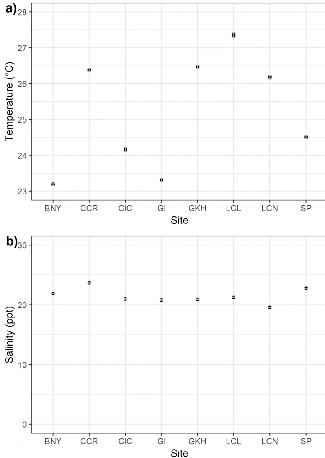
Figure 36. A) Average temperature in July 2018, and B) average salinity (ppt) across 2018 from high-resolution (recorded every 15 minutes) data for Brooklyn Navy Yard (BNY), Canarsie Community Reef (CCR), Coney Island Community Reef (CIC), Governors Island EcoDock (GI), Great Kills Harbor (GKH), Lemon Creek Lagoon (LCL), Lemon Creek Nursery (LCN), and Sunset Park Community Reef (SP). Error bars represent 95% confidence intervals.
