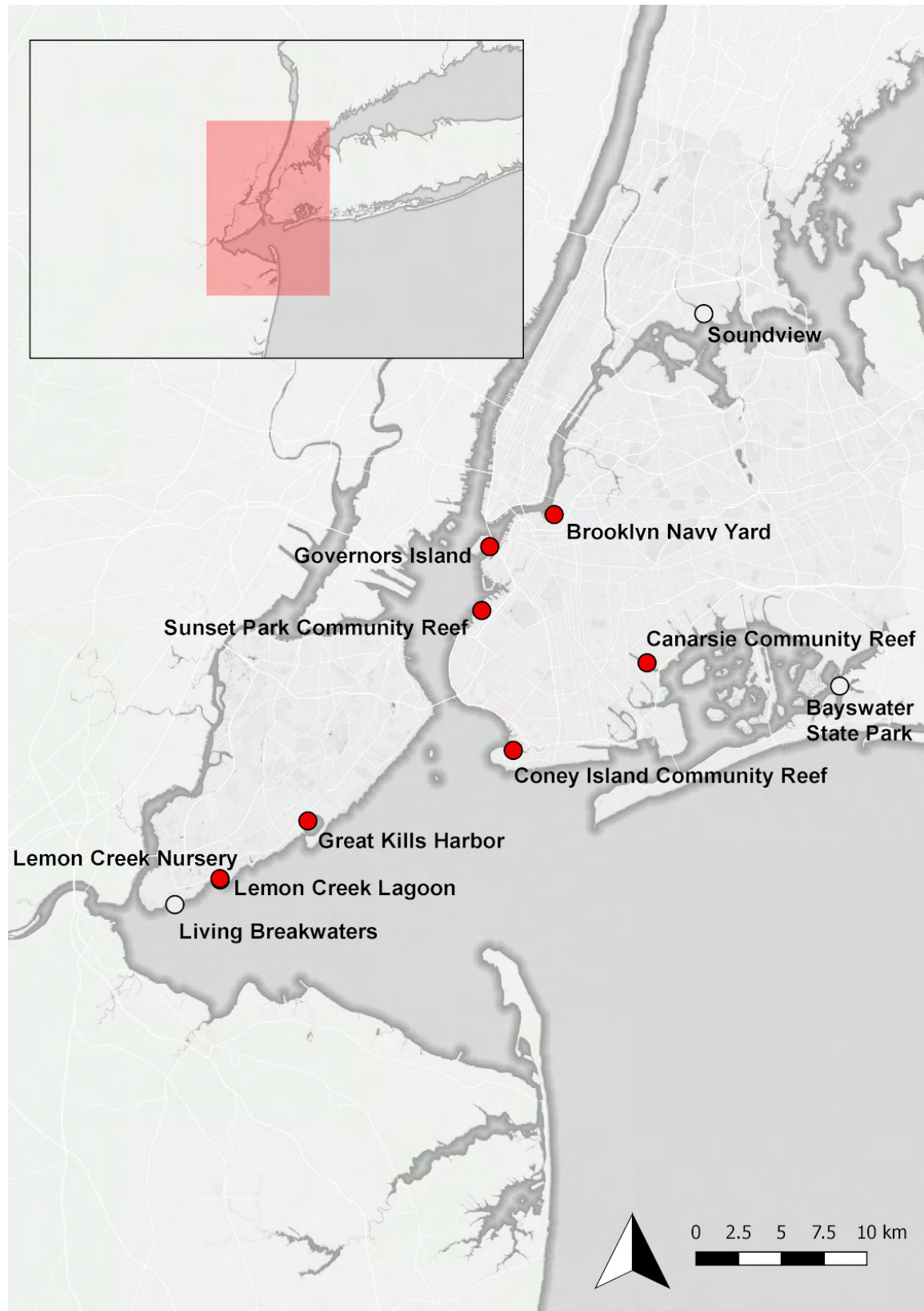
Figure 3. The eight current oyster restoration sites in New York Harbor described in this document are represented by red circles. The three future restoration sites are indicated with white circles.
