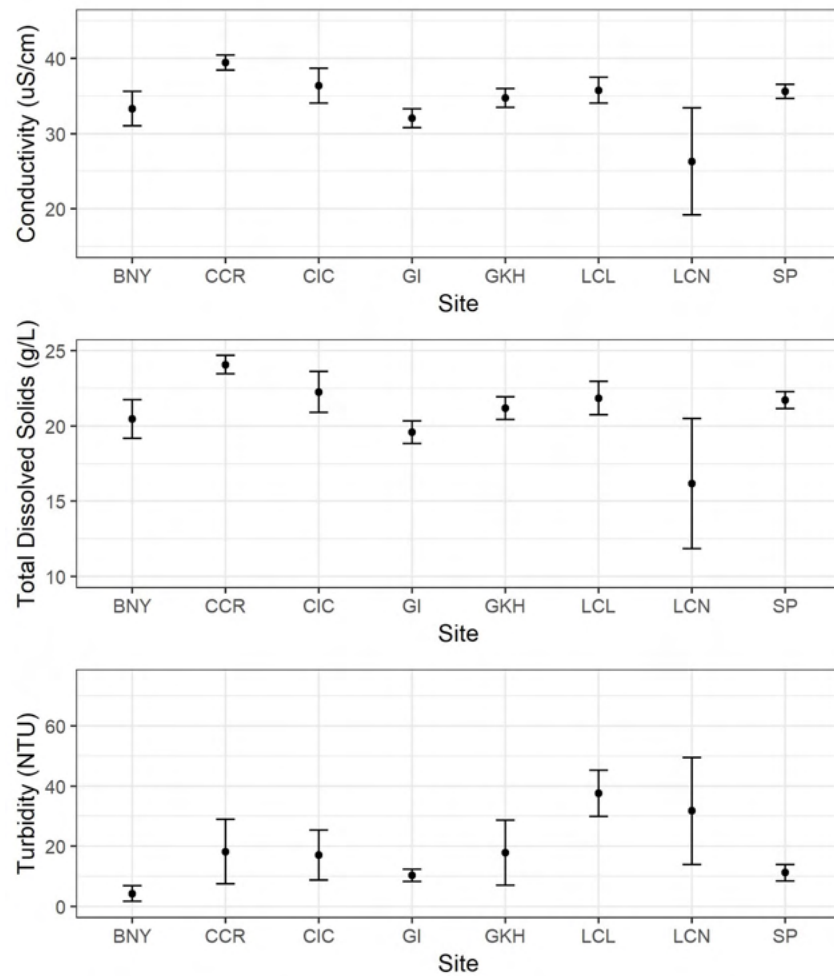
Figure 34. Average values of conductivity, total dissolved solids, and turbidity from June through September 2018, based on discrete point sampling for Brooklyn Navy Yard (BNY) (n = 3), Canarsie Community Reef (CCR) (n = 4), Coney Island Community Reef (CIC) (n = 5), Governors Island (GI) EcoDock (n = 6), Great Kills Harbor (GKH) (n = 4), Lemon Creek Lagoon (LCL) (n = 5), Lemon Creek Nursery (LCN) (n = 4), and Sunset Park (SP) Community Reef (n = 4). Error bars represent 95% confidence intervals.
