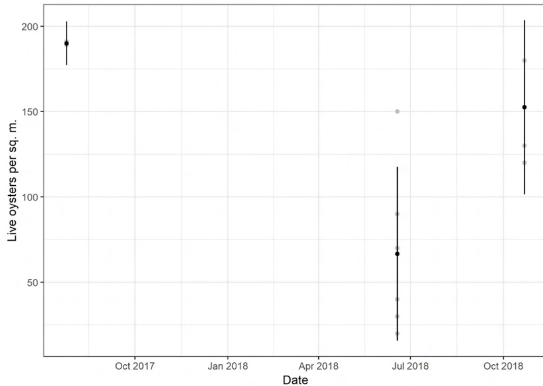
Figure 20. Oyster density (live oysters per square meter) at the Sunset Park Community Reef installed in 2016. Grey points represent individual data points. Black points are average values for each date. Error bars represent 95% confidence intervals.
