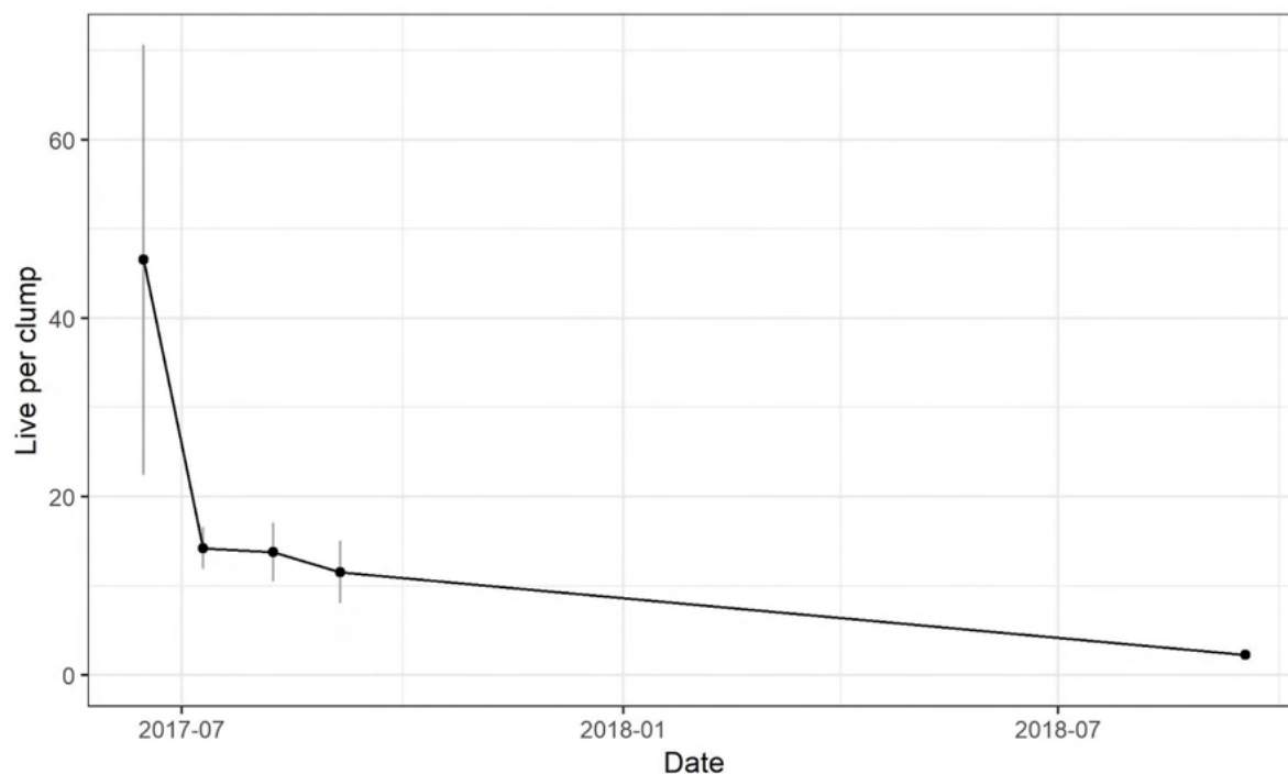
Figure 18. Oyster density (i.e., live oysters per clump) declined over time in Oyster Gros at the Lemon Creek Nursery (LCN) in 2017 and 2018. Error bars represent 95% confidence intervals.
