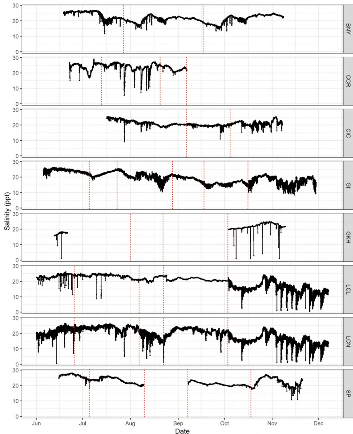
Figure 37. High-resolution (recorded every 15 minutes) salinity data for Brooklyn Navy Yard (BNY), Canarsie Community Reef (CCR), Coney Island Community Reef (CIC), Governors Island EcoDock (GI), Great Kills Harbor (GKH), Lemon Creek Lagoon (LCL), Lemon Creek Nursery (LCN), and Sunset Park Community Reef (SP). Red lines indicate dates when loggers were cleaned, calibrated, and redeployed.
