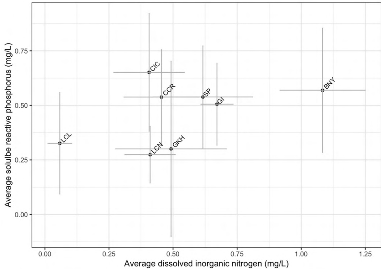
Figure 45. Average soluble reactive phosphorus concentration and dissolved inorganic nitrogen (nitrite, nitrate, and ammonium) in 2018 at Brooklyn Navy Yard (BNY), Canarsie Community Reef (CCR), Coney Island Creek Community Reef (CIC), Governors Island (GI) EcoDock, Great Kills Harbor (GKH), Lemon Creek Lagoon (LCL), Lemon Creek Nursery (LCN), and Sunset Park (SP) Community Reef in 2018. Error bars represent 95% confidence intervals.
