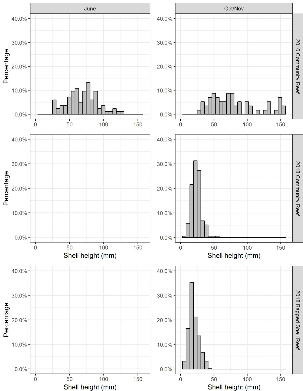
Figure 15. Size frequency distribution of oyster shell heights at Sunset Park in the 2016 community reef (top row), 2018 community reef (middle row), and 2018 bagged shell reef (bottom row) in June and October/November 2018.
