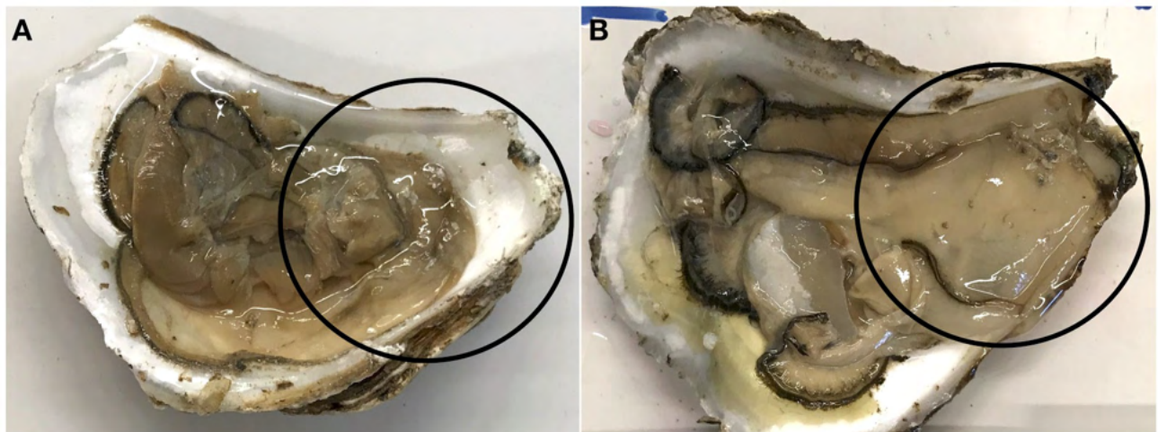
Figure 25. These pictures compare gonad development (circled) in (A) inactive or “unripe” and (B) “ripe” oyster tissue.
