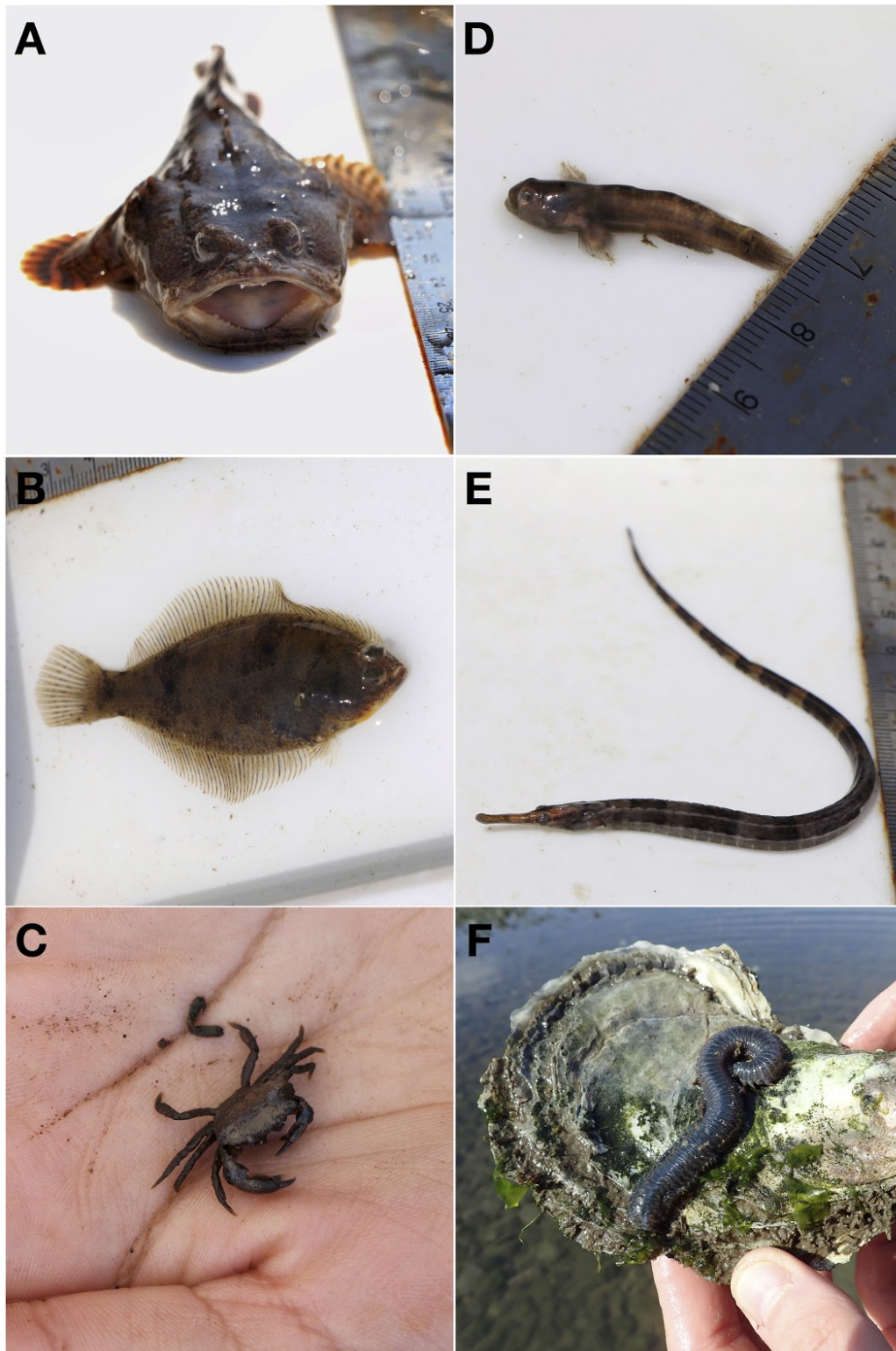
Figure 47. Examples of organisms inhabiting restored reefs: (A) Oyster toadfish ( Opsanus tau ), (B) Winter flounder ( Pseudopleuronectes americanus ), (C) Mud crab ( Panopeus sp.), (D) Naked goby ( Gobiosoma bosc ), (E) Northern pipefish ( Sygnathus fuscus ), and (F) Clam worm ( Nereis sp.).
