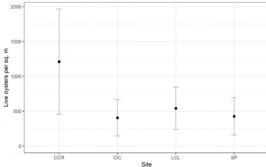
Figure 19. Oyster density (live oysters per square meter) at community reefs and gabions that were newly installed in 2018 (CCR: Canarsie Community Reef, CIC: Coney Island Community Reef, LCL: Lemon Creek Lagoon, SP: Sunset Park Community Reef). Oysters were deployed between July 12 and August 21, 2018, and oyster measurements were taken between October 22 and December 6, 2018. Error bars represent 95% confidence intervals.
