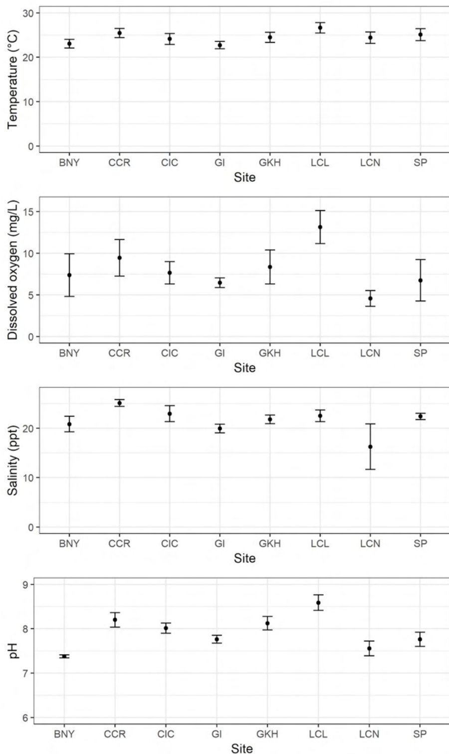
Figure 33. Average values of temperature, dissolved oxygen, salinity, and pH from June through September 2018, based on discrete point sampling for Brooklyn Navy Yard (BNY) (n = 3), Canarsie Community Reef (CCR) (n = 4), Coney Island Community Reef (CIC) (n = 5), Governors Island (GI) EcoDock (n = 6), Great Kills Harbor (GKH) (n = 4), Lemon Creek Lagoon (LCL) (n = 5), Lemon Creek Nursery (LCN) (n = 4), and Sunset Park (SP) Community Reef (n = 4). Error bars represent 95% confidence intervals.
