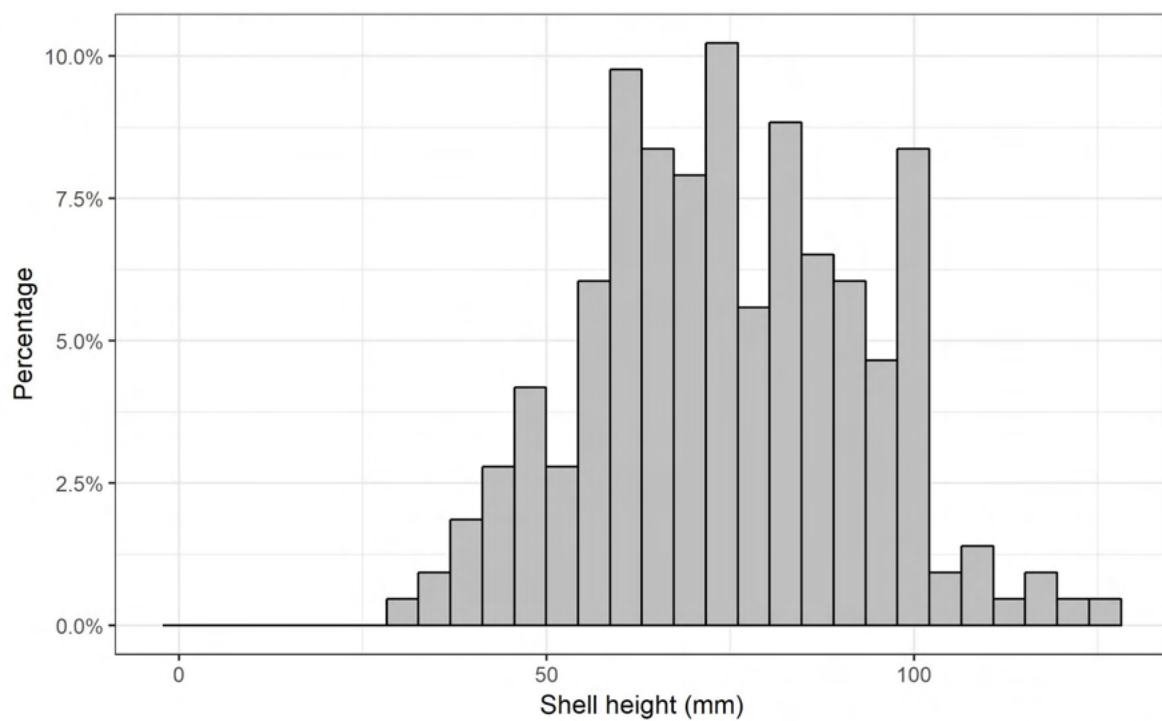
Figure 13. Size frequency distribution of live oyster shell heights at Lemon Creek Nursery in September 2018.
