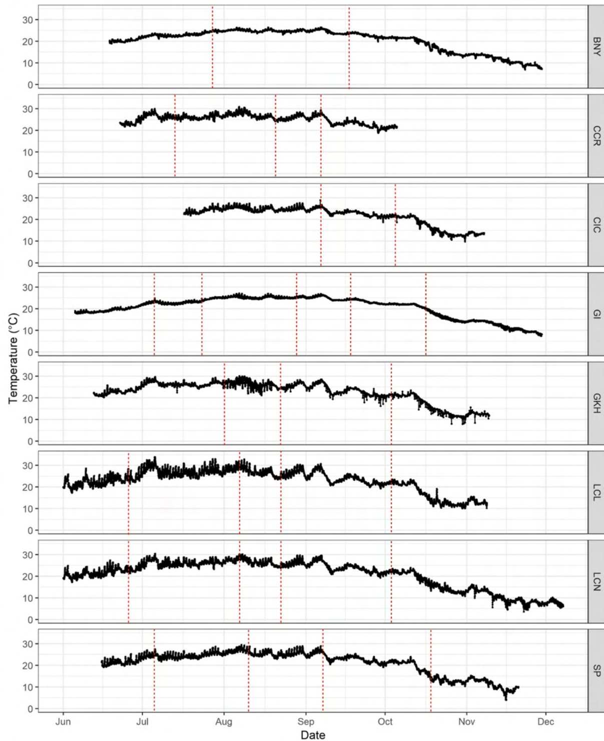
Figure 35. High-resolution (recorded every 15 minutes) temperature data for Brooklyn Navy Yard (BNY), Canarsie Community Reef (CCR), Coney Island Community Reef (CIC), Governors Island EcoDock (GI), Great Kills Harbor (GKH), Lemon Creek Lagoon (LCL), Lemon Creek Nursery (LCN), and Sunset Park Community Reef (SP). Red lines indicate dates when loggers were cleaned, calibrated, and redeployed.
