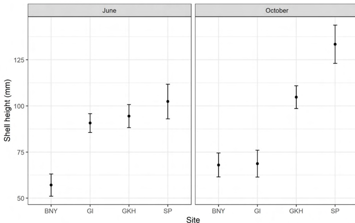
Figure 23. Shell heights of oysters sampled from Brooklyn Navy Yard (BNY), Governors Island EcoDock (GI), Great Kills Harbor (GKH) MBSOS07152015 cohort installed in 2016, and the Sunset Park (SP) Community Reef in June and October (n = 30 oysters from each site, except n = 27 for SP). Error bars represent 95% confidence intervals.
