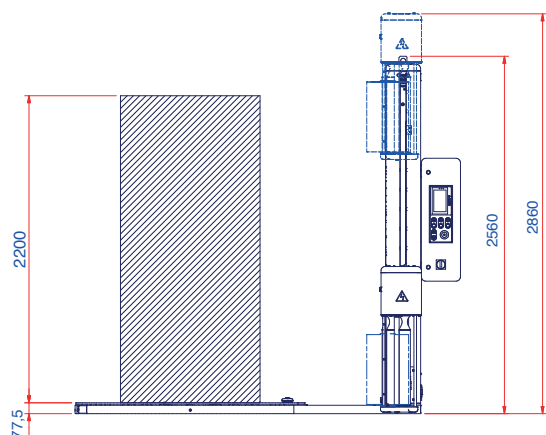
LAYOUT ROTOPLAT 708 PVS [mm]
