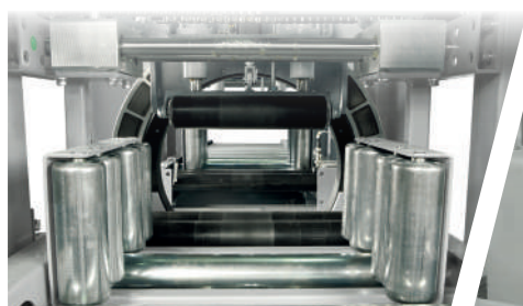
GUIDE LATERALI A RULLI IN ENTRATA E USCITA / INCOMING AND OUTGOING SIDE ROLLER GUIDES
