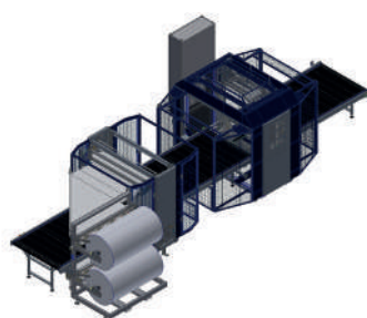
BOBINE LATERALI LATERAL REEL
