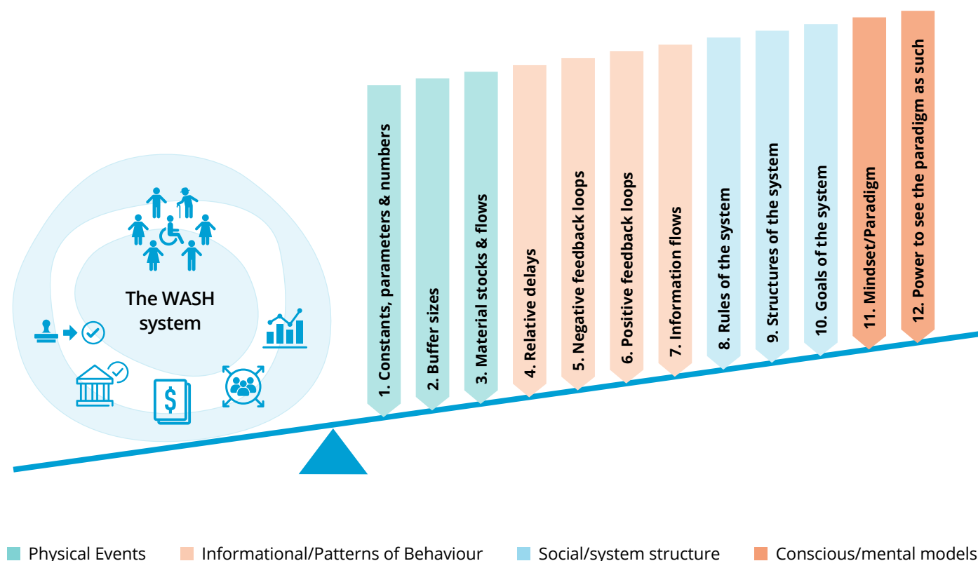
Figure 2. Donella Meadows’ leverage points
