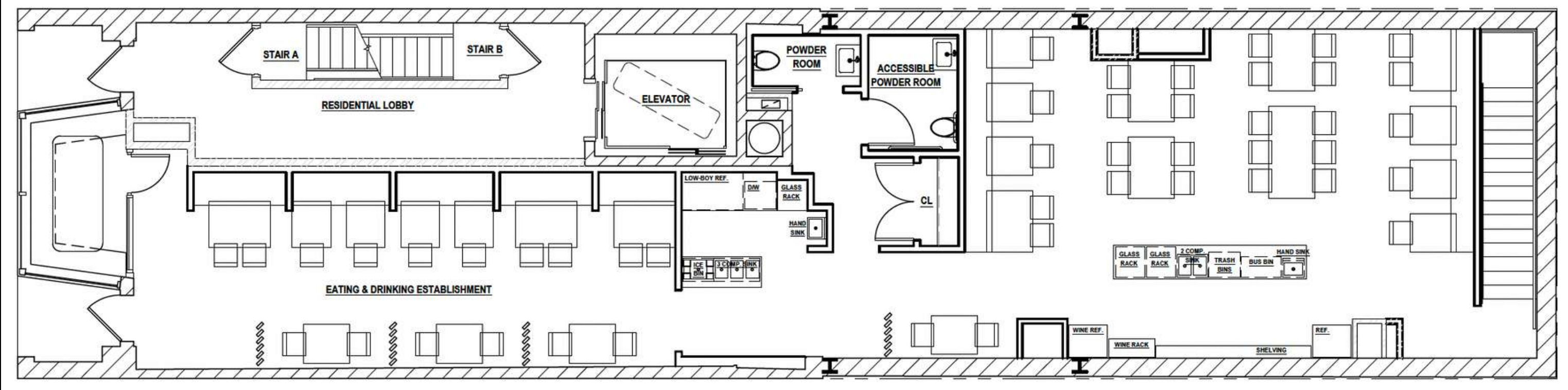
GROUND FLOOR
