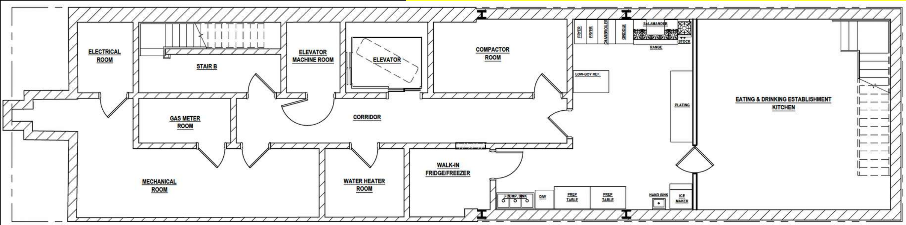
LOWER LEVEL
