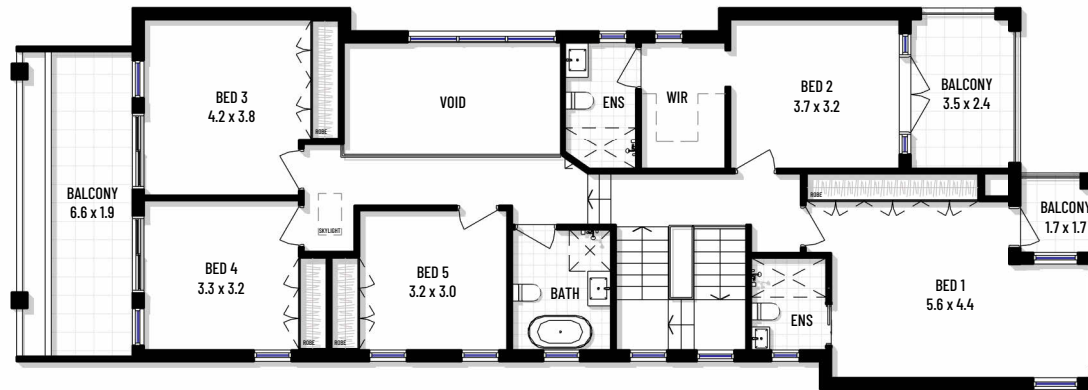
FIRST LEVEL
