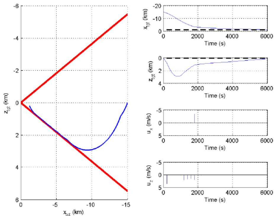
Figure 11.26: Behavior with cost given by 1-norm.
