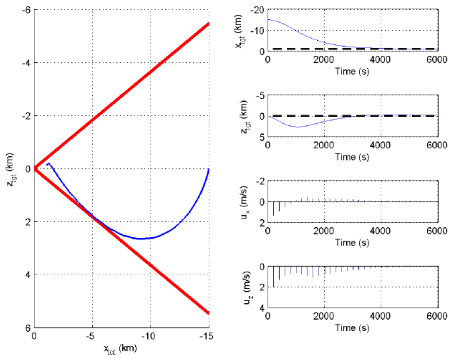
Figure 11.25: Behavior with quadratic cost.
