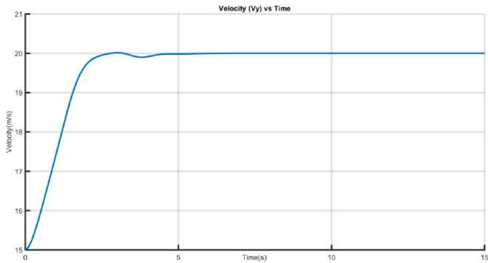
Figure 7.7: Vehicle velocity.
