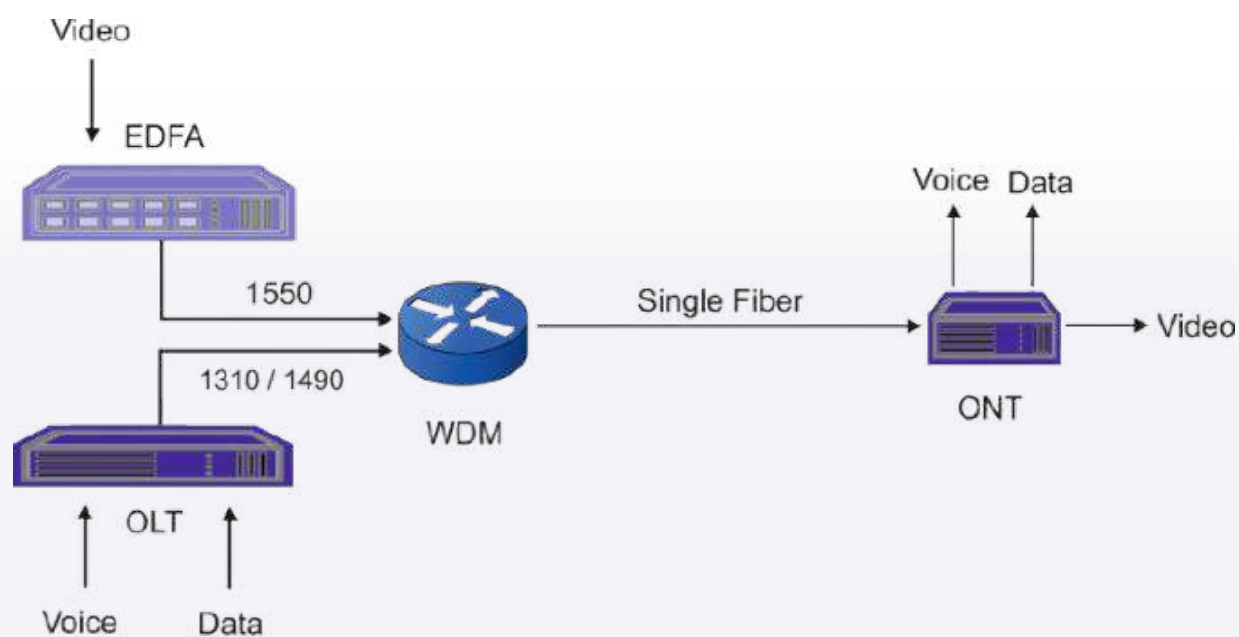
GPON Solution
