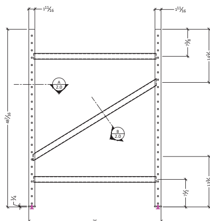
1 Widespan Upright Post - SideView 2.0 SCALE: 1" = 1'-0"
