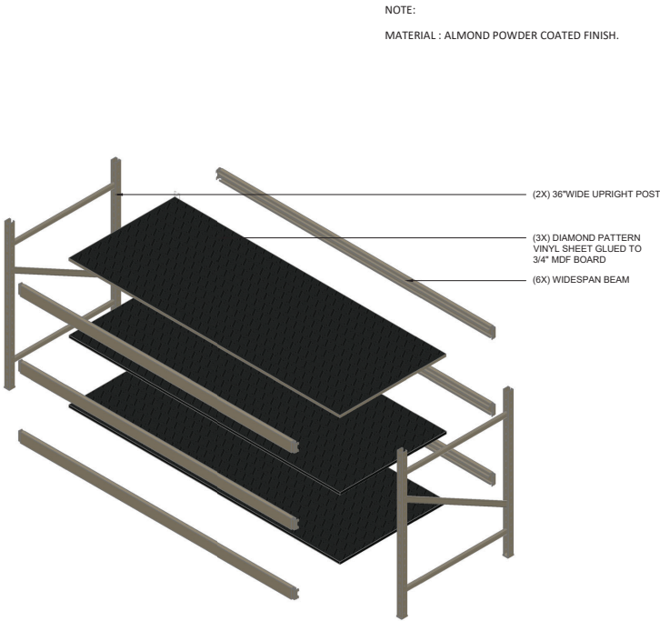
EXPLODED VIEW
