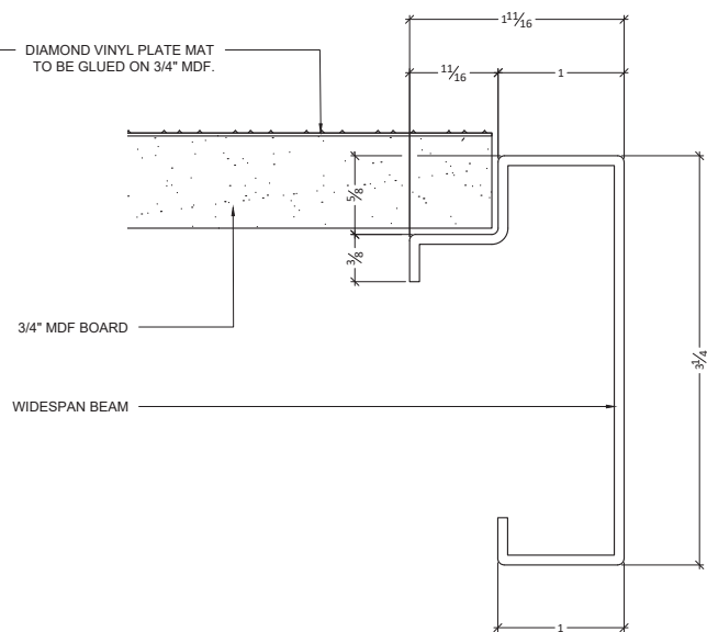
SHELF DETAIL SECTION
