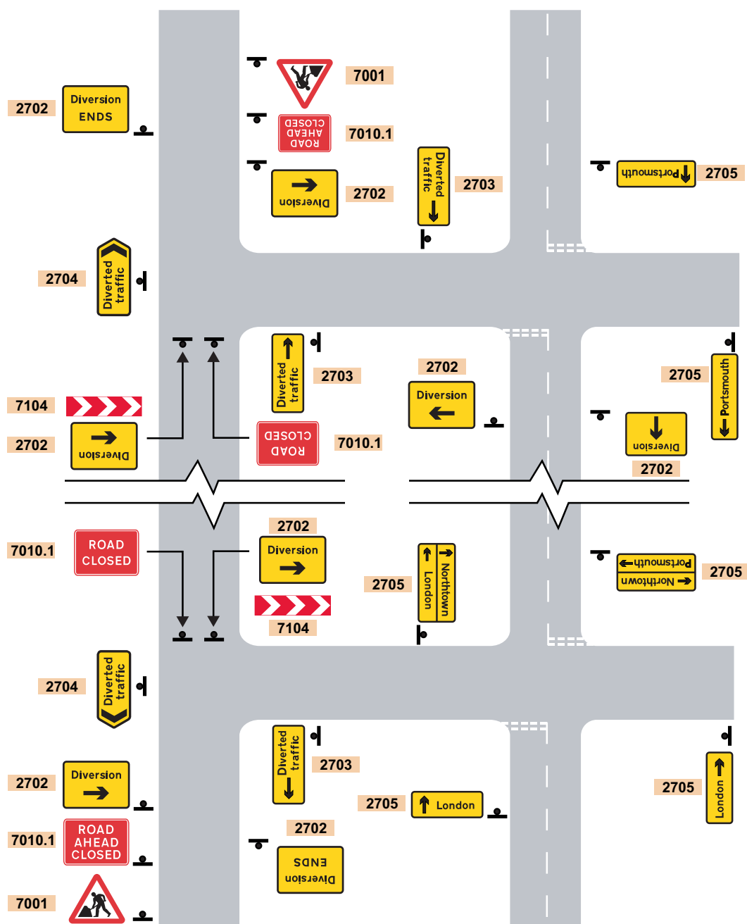
Figure 3.3 Layout of signs for road works on single carriageway roads with diversions
