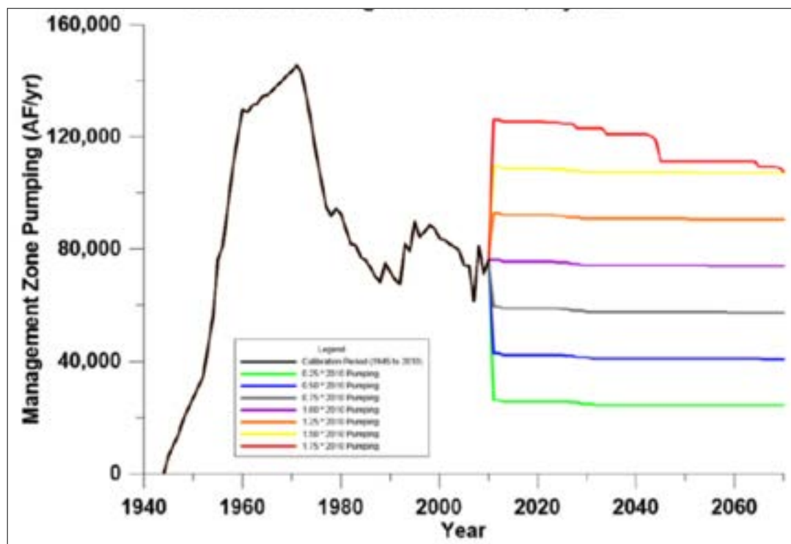
Figure 9.2: Historical pumping in the Harden and others (2011) model for Management Zone 1 (black line) and seven scenarios of projected pumping (colored lines; from Hutchison 2017b).
