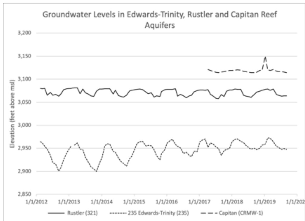
Figure 4.7: Groundwater levels in Edwards-Trinity, Rustler, and Capitan Reef aquifers (data from the Middle Pecos Groundwater Conservation District; msl = mean sea level).
