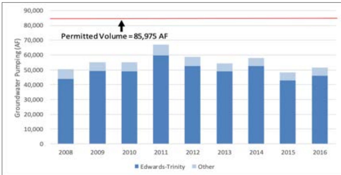
Figure 10.2: Permitted volume and annual groundwater use in Management Zone 1 from 2008 through 2016 (data from the Middle Pecos Groundwater Conservation District).
