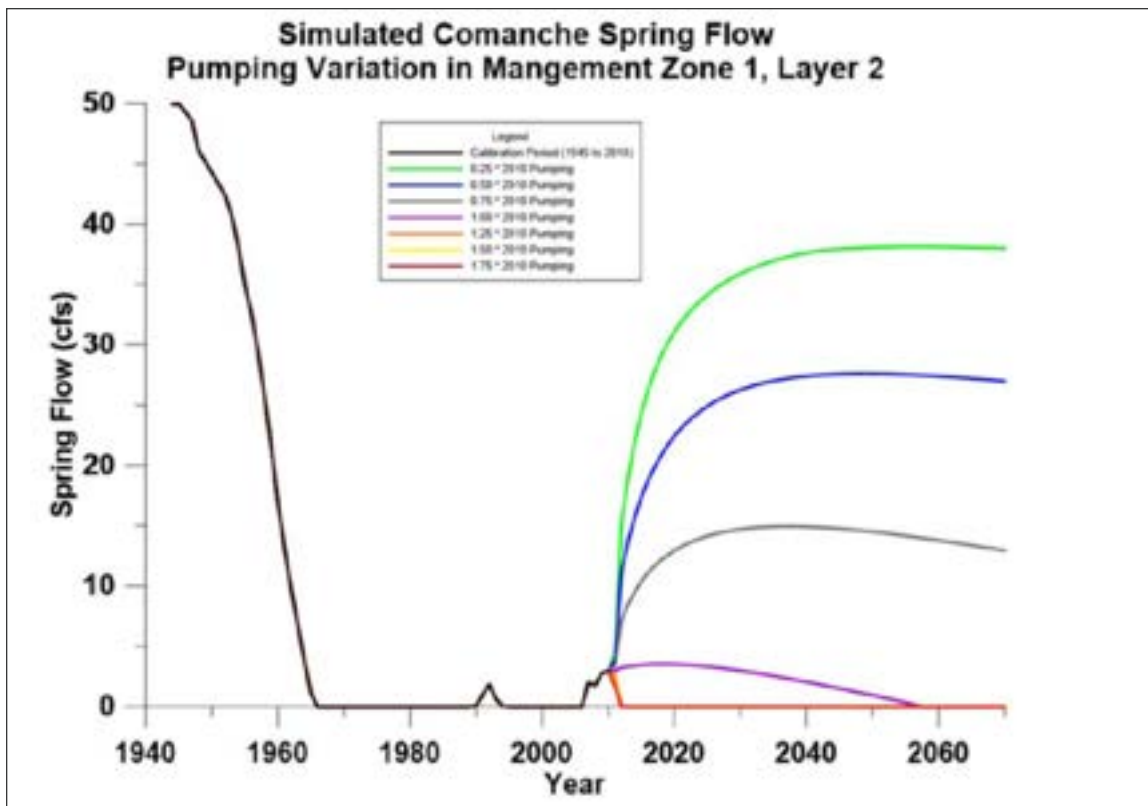
Figure 9.3: Simulated flow at Comanche Springs for the historical pumping in the Harden and others (2011) model for Management Zone 1 (black line) and for seven scenarios of projected pumping (colored lines; from Hutchison 2017b; see Figure 9.1 for the pumping scenarios).
