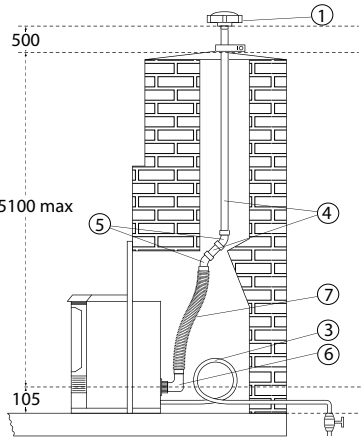
Masonry Internal
