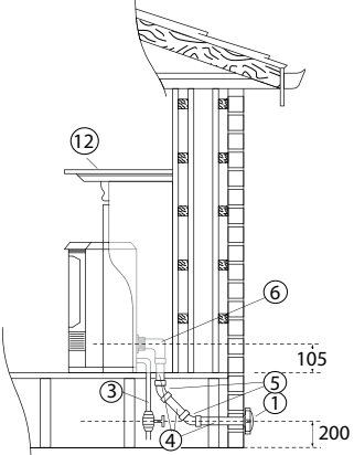
Under Floor
