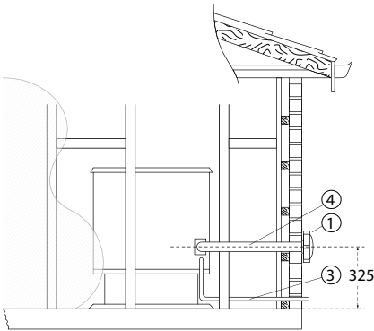
External Wall
