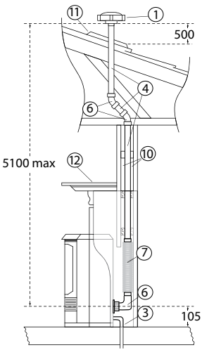
Masonry Internal
