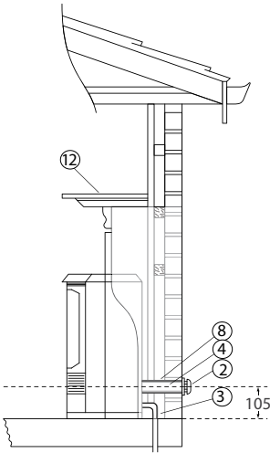
Masonry External
