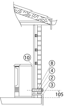
External Wall
