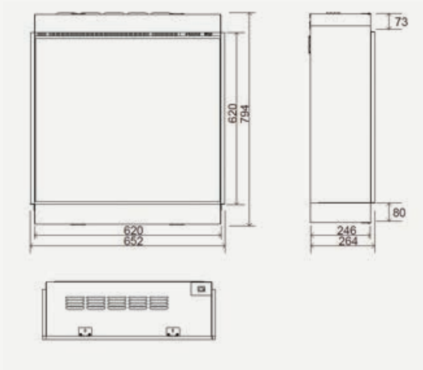
LUMINOSA 62 - OVERALL UNIT DIMENSIONS (MM)
