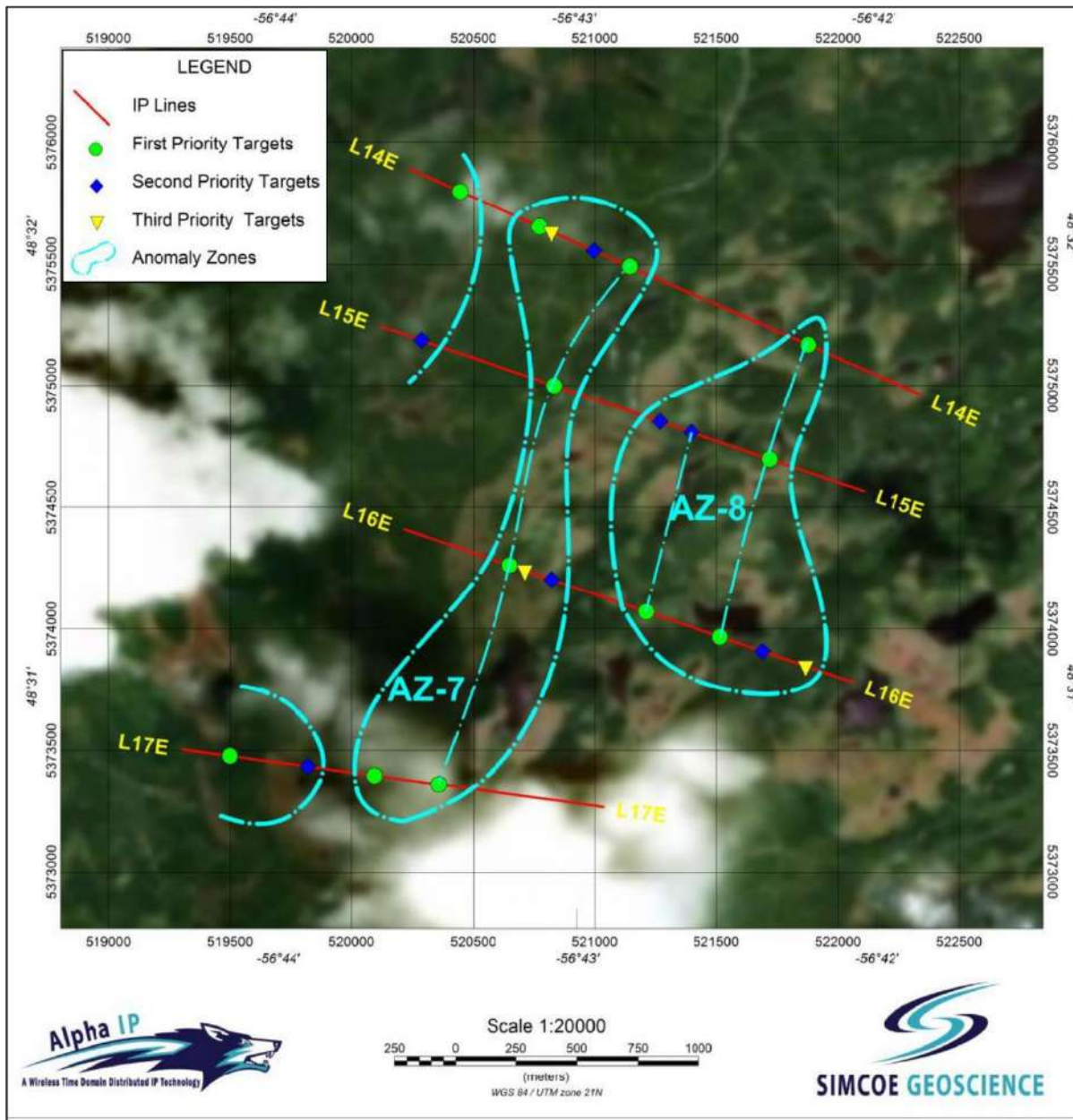
Figure 24. IP survey lines Lemarchant Property. Also shown are anomalies and priority targets (from Mirza, 2022).
