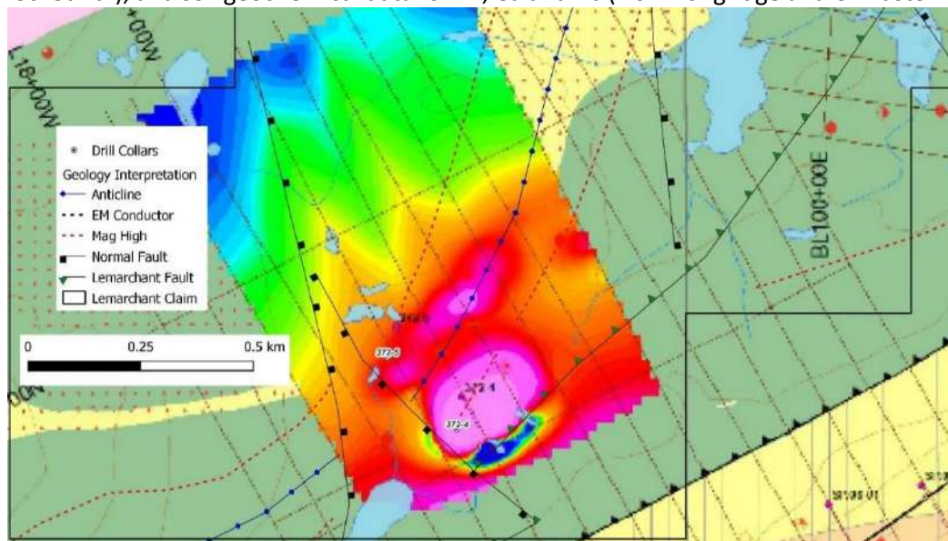
Figure 19. Results of a 2016 PEM survey over the Southwestern Target (from Longridge and Chrzastowski, 2023).
