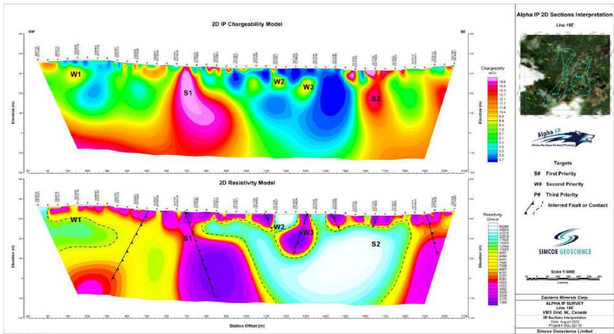
Figure 26. Lemarchant - Line 15E Interpreted Chargeability and Resistivity Sections (from Mirza, 2022).
