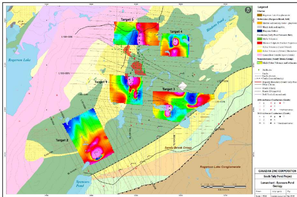
Figure 9. 2016 PEM and 2017 TDEM Survey Areas - Targets 1-5 (from Cullen et al., 2018).
