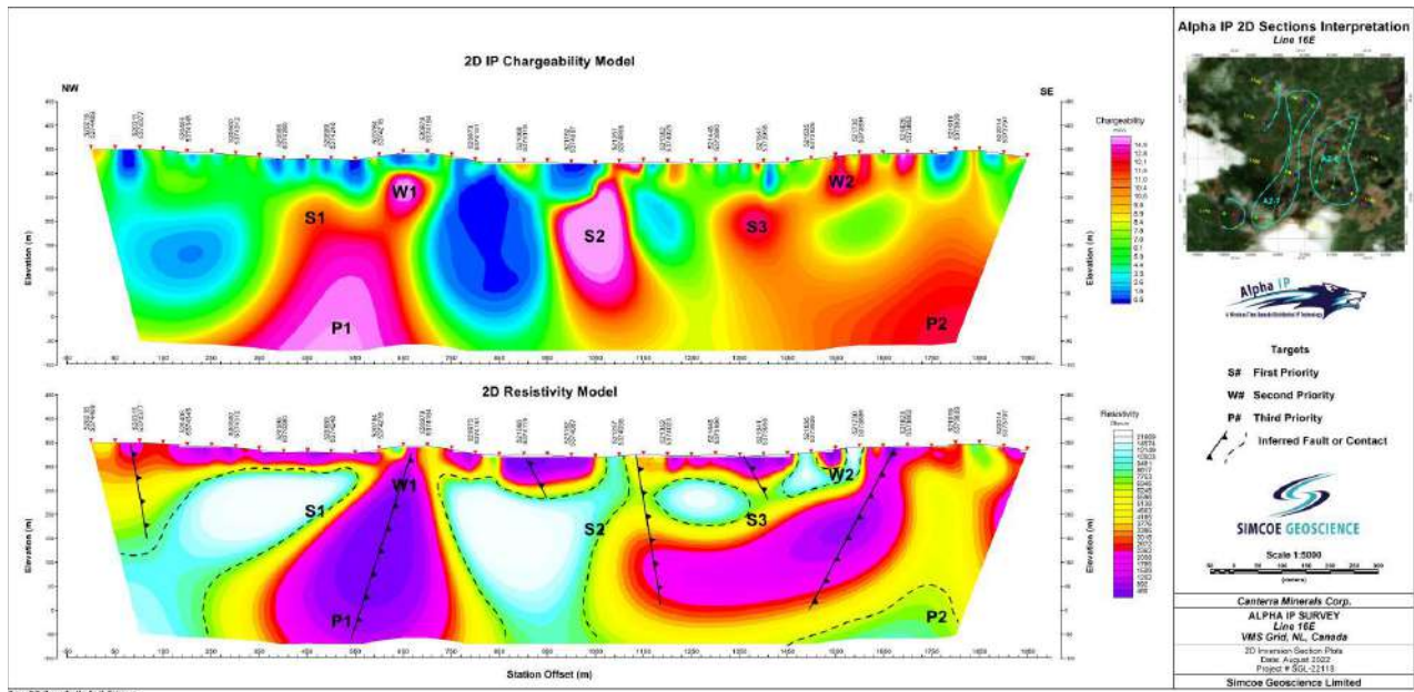
Figure 27. Lemarchant - Line 16E Interpreted Chargeability and Resistivity Sections (from Mirza, 2022).
