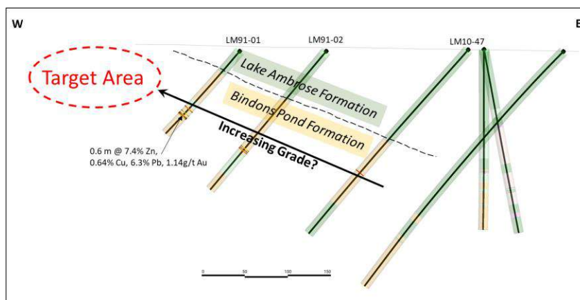
Figure 21. East-west cross section south of the Main Zone - note the possible increase in grade (and thickness) of mineralization towards the west (from Longridge and Chrzastowski, 2023).
