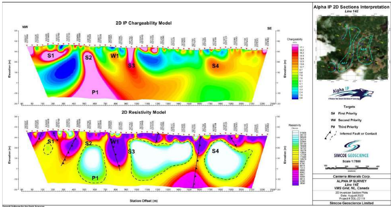
Figure 25. Lemarchant - Line 14E Interpreted Chargeability and Resistivity Sections (from Mirza, 2022).
