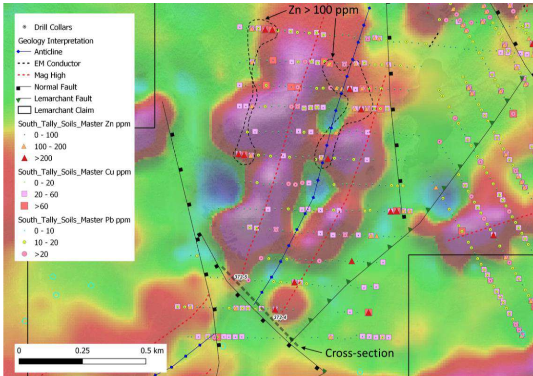
Figure 18. Map of the Southwest Target, showing the location of the cross-section ( Error! Reference source not found. ), and soil geochemical data for Zn, Cu and Pb (from Longridge and Chrzastowski, 2023).
