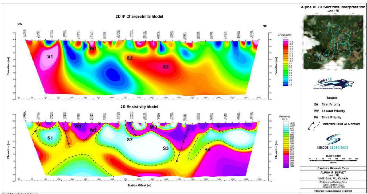
Figure 28. Lemarchant - Line 17E Interpreted Chargeability and Resistivity Sections (from Mirza, 2022).
