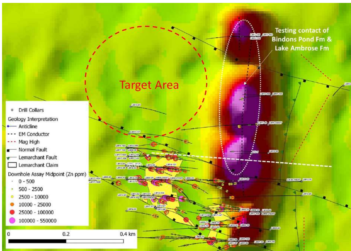
Figure 23. Map of the Northwest Zone Extension Target (from Longridge and Chrzastowski, 2023). Base Map are airborne EM anomalies (2011). Note that the Northwest Zone has no EM response, and that the contact between the Bindons Pond Formation and the Lake Ambrose Formation is marked by a graphitic mudstone horizon that gives a strong EM response.
