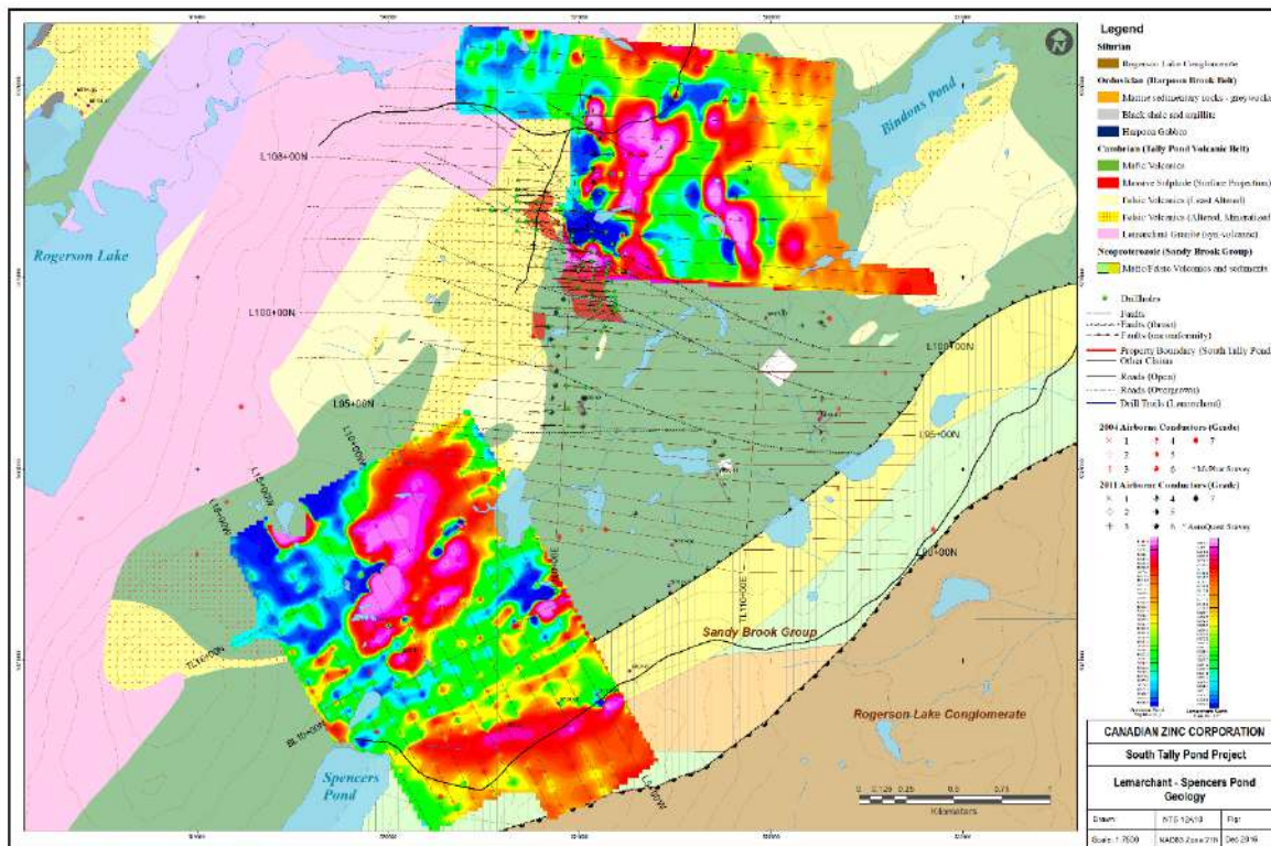
Figure 5. 2016 Magnetic Survey Data (from Cullen et al., 2018).
