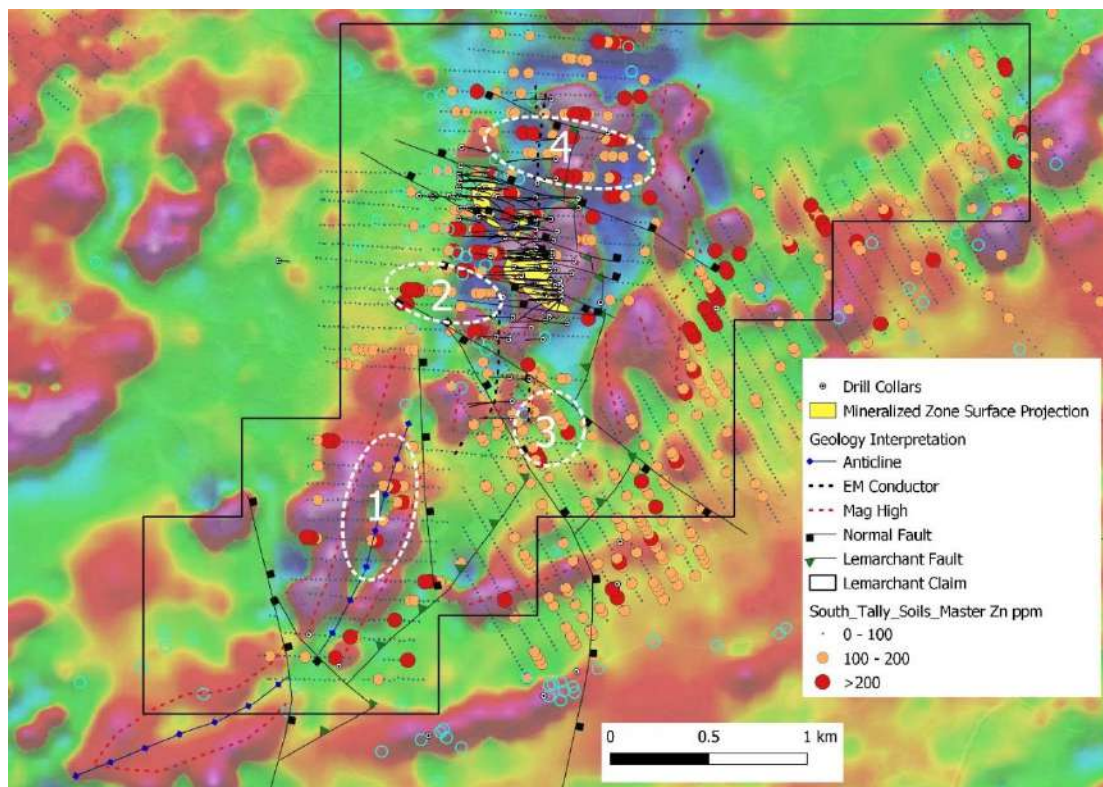
Figure 16. Lemarchant Project structural interpretation based on airborne magnetic data, Zn soils and deposit locations (from Longridge and Chrzastowski, 2023).
