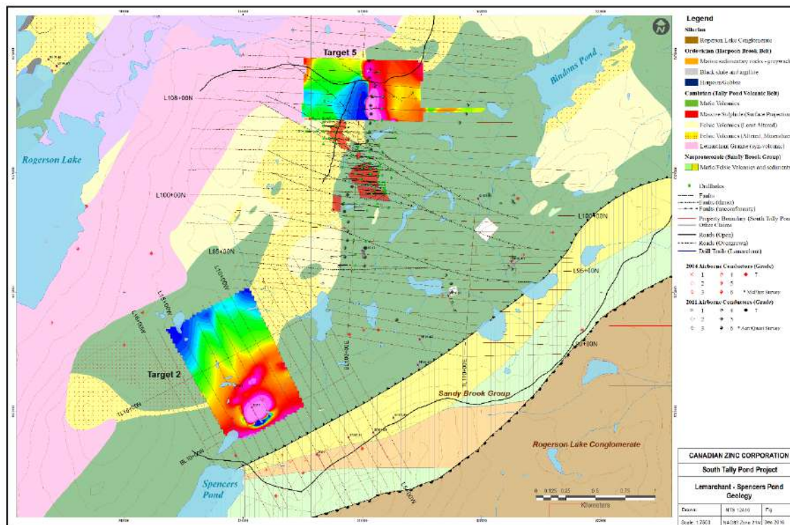
Figure 8. 2016 PEM Survey Areas - Targets 2 and 5 (from Cullen et al., 2018).
