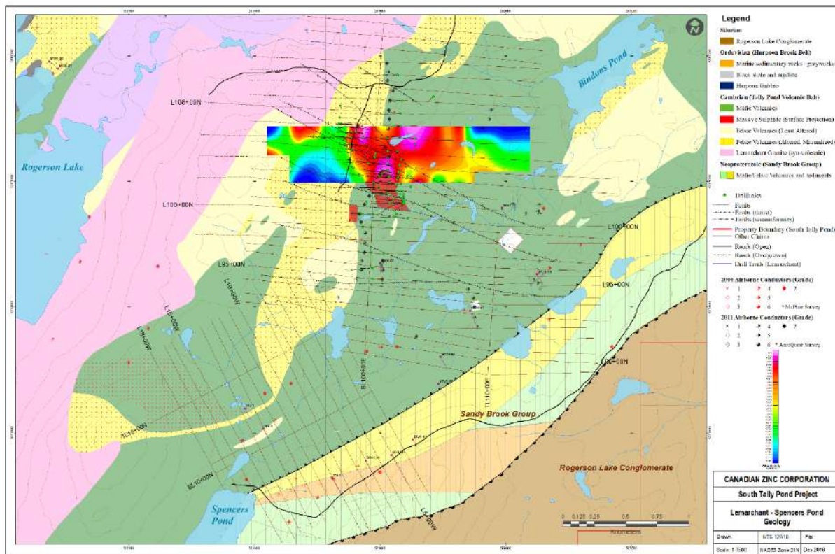
Figure 4. 2014 Orientation Gravity Survey (from Cullen et al., 2018).
