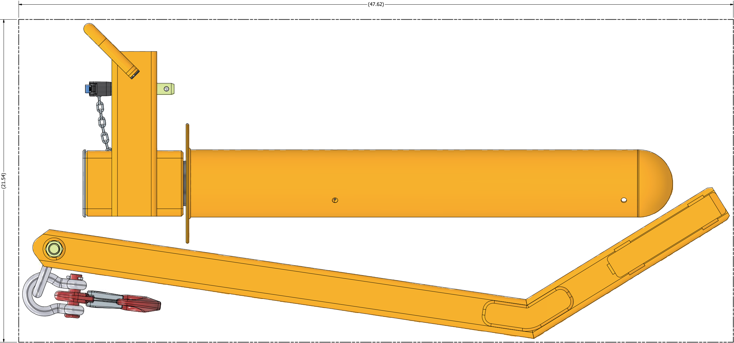
PACK AND SHIP ORIENTATION
